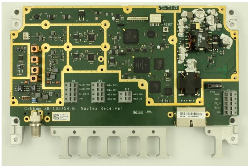
COVER & RF SHIELD DISMOUNTED
