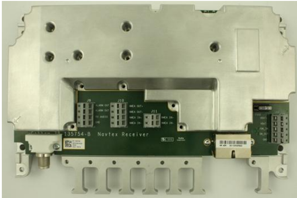
COVER DISMOUNTED & RF SHIELD MOUNTED
