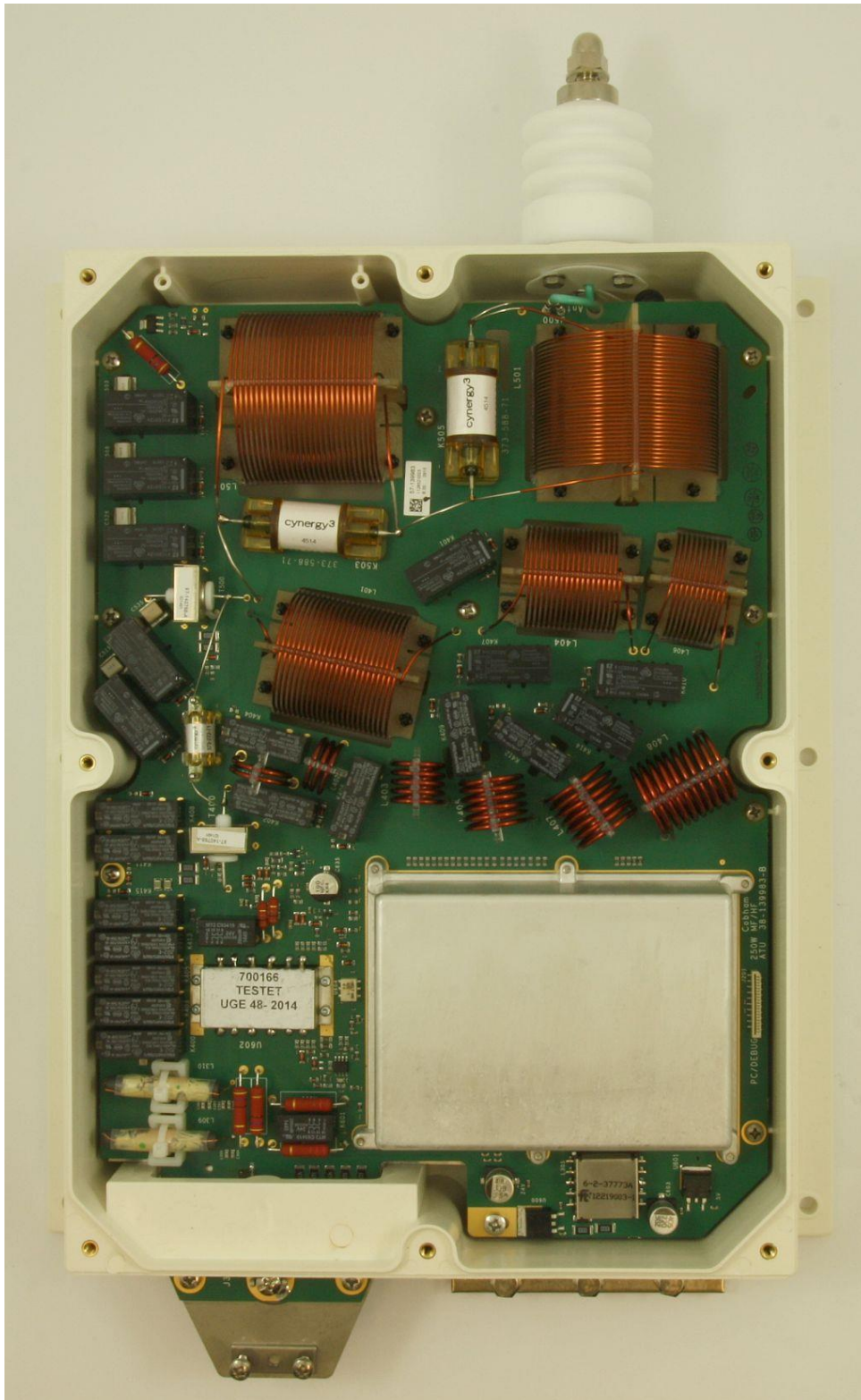
SAILOR 6384 lid off
