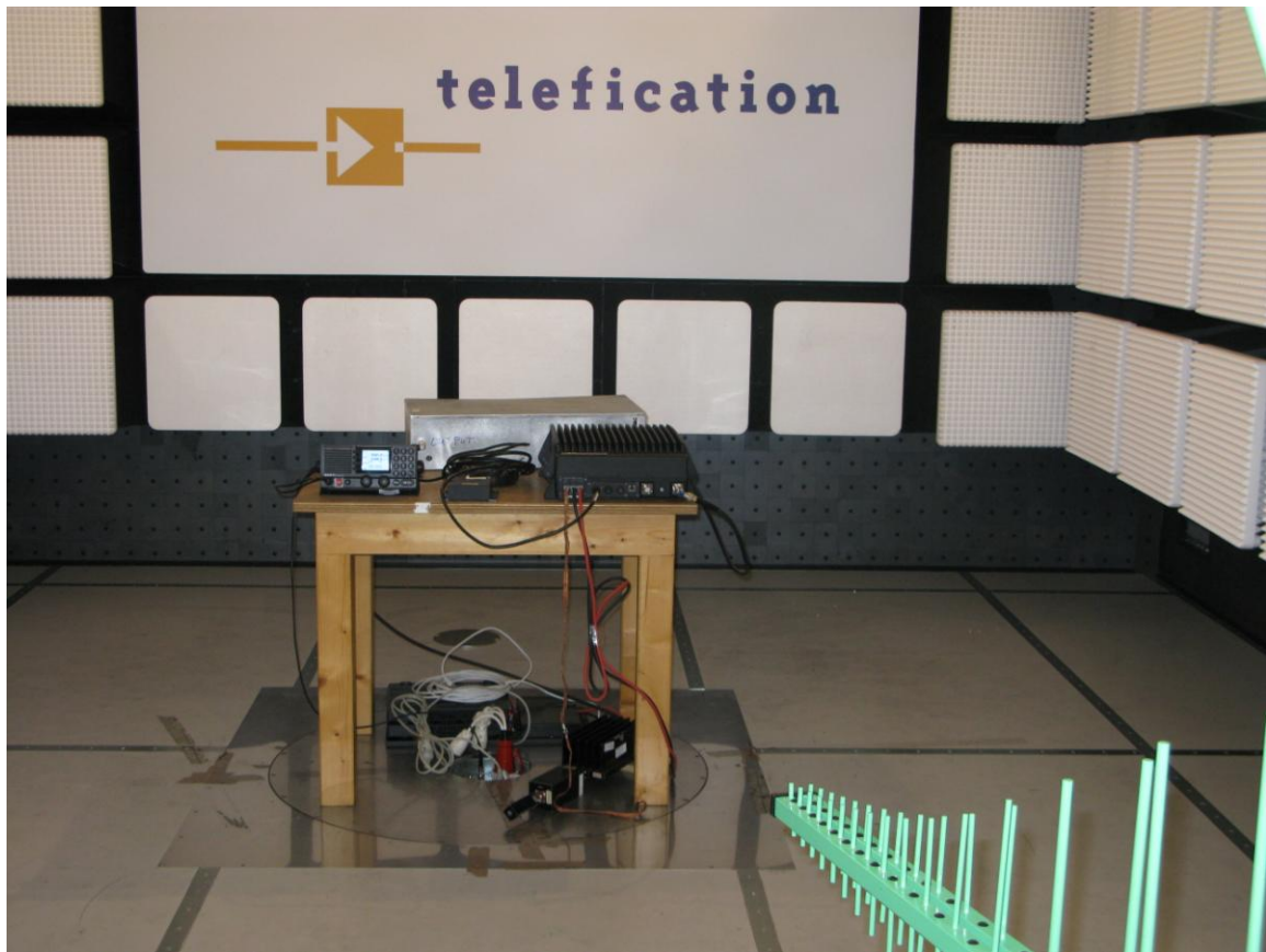
Photograph 2: Test setup radiated emissions (0.03 - 1 GHz)
