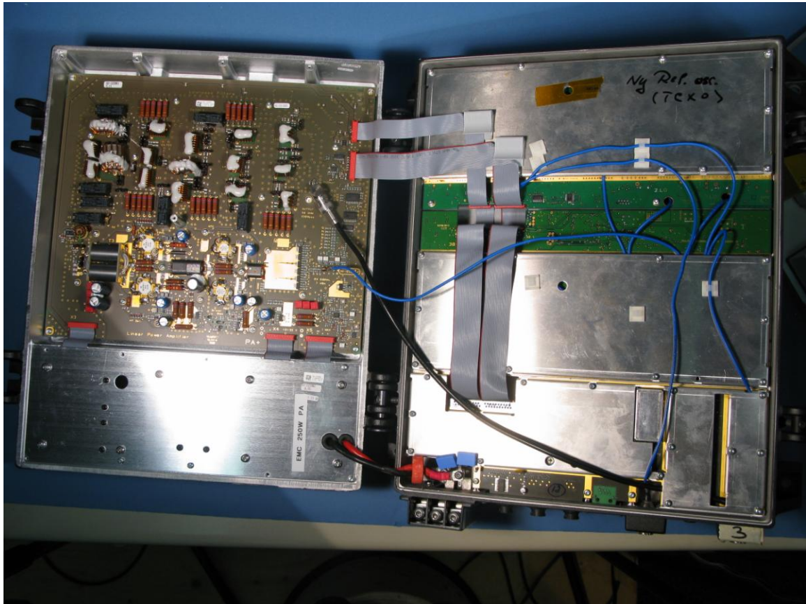
Photograph 1: Transceiver unit, internal view
