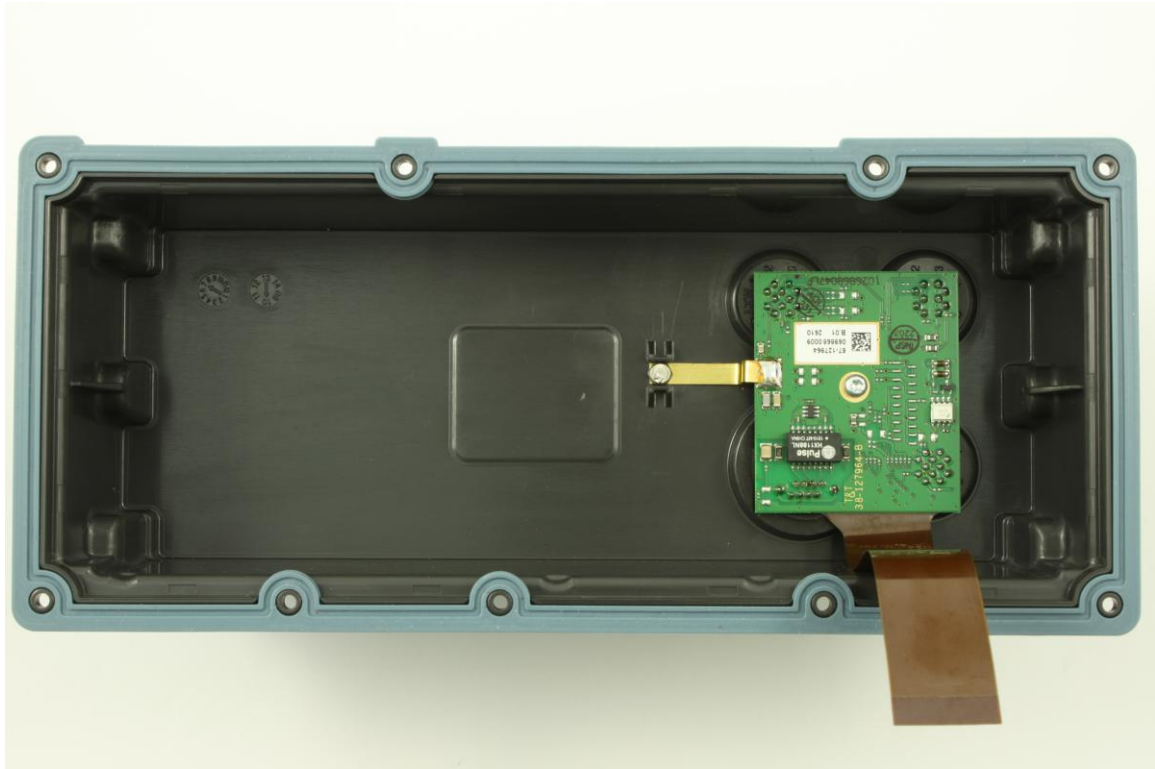
Photograph 3: Control unit, rear seen from the inside
