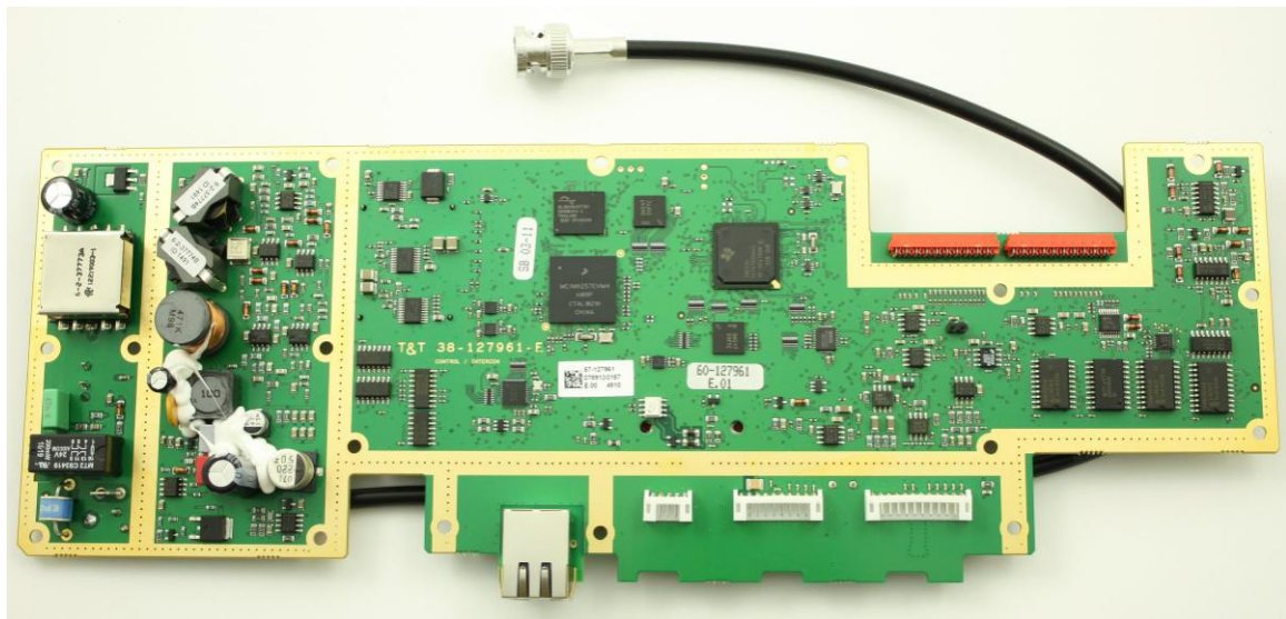
Photograph 5: Control unit, PCB top view
