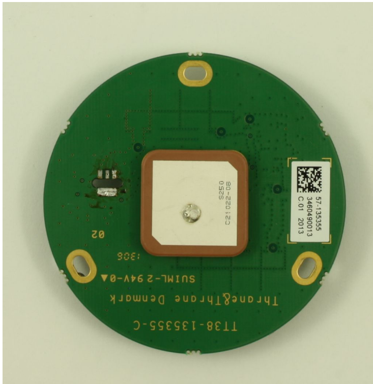
SAILOR 6285 pcb top view
