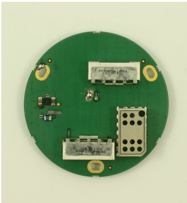
SAILOR 6285 pcb bottom view
