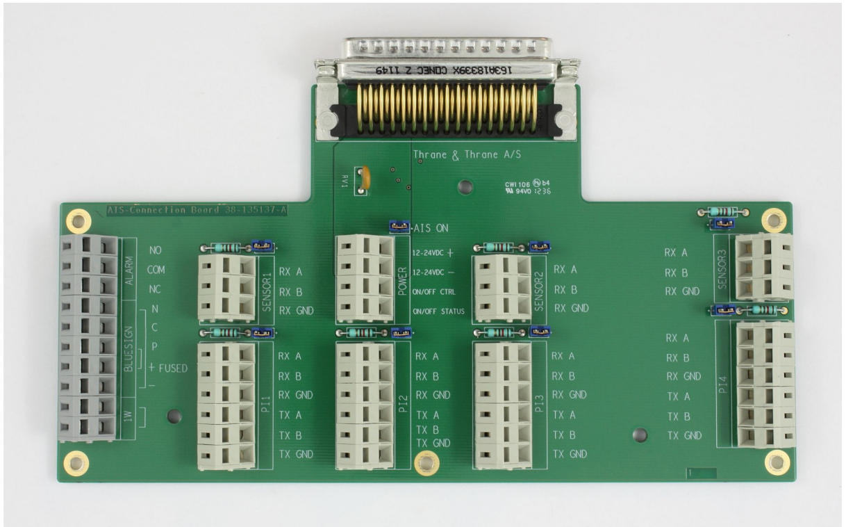
SAILOR 6283 pcb top view
