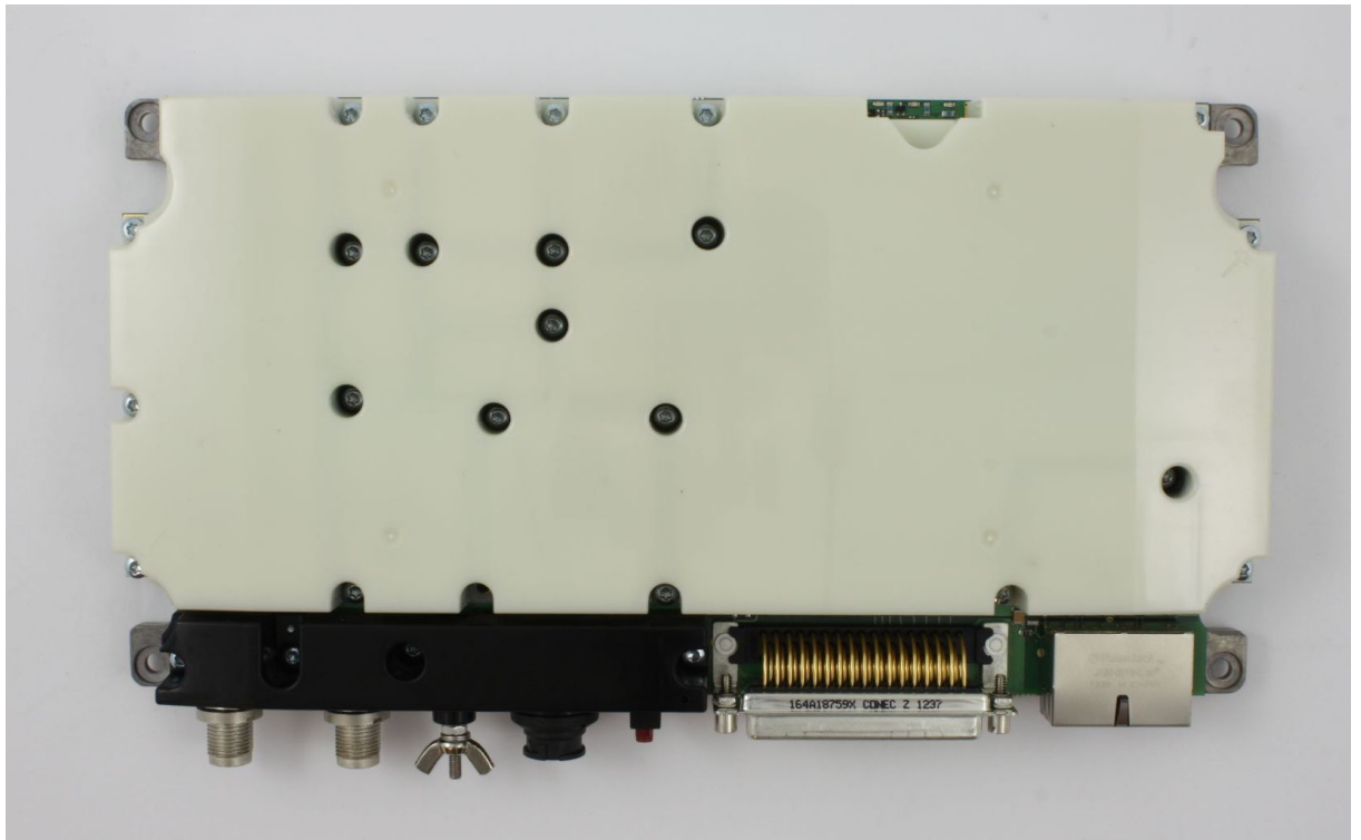
SAILOR 6282 with cover off and rf screen
