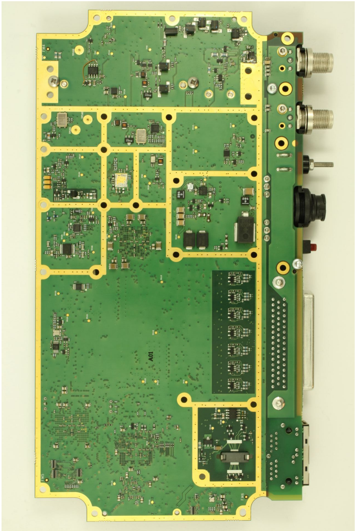
SAILOR 6282 pcb bottom
