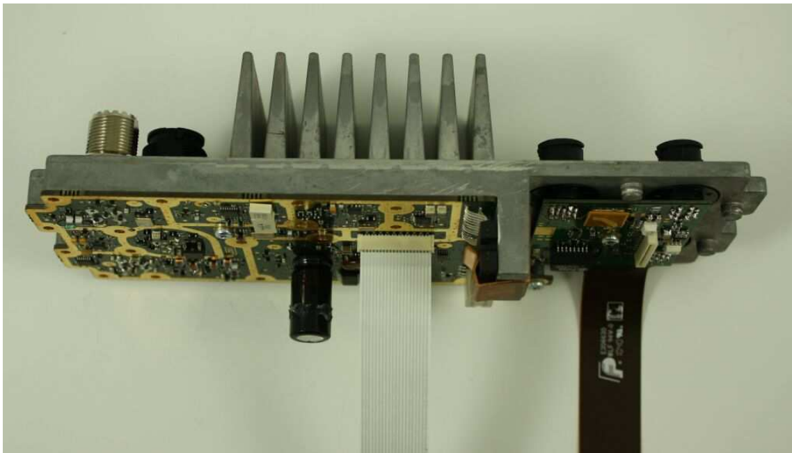
Main unit without housing -2
