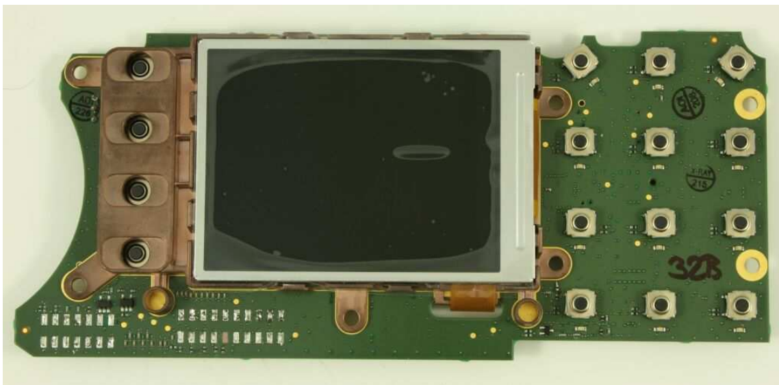
Control – Display modules back view
