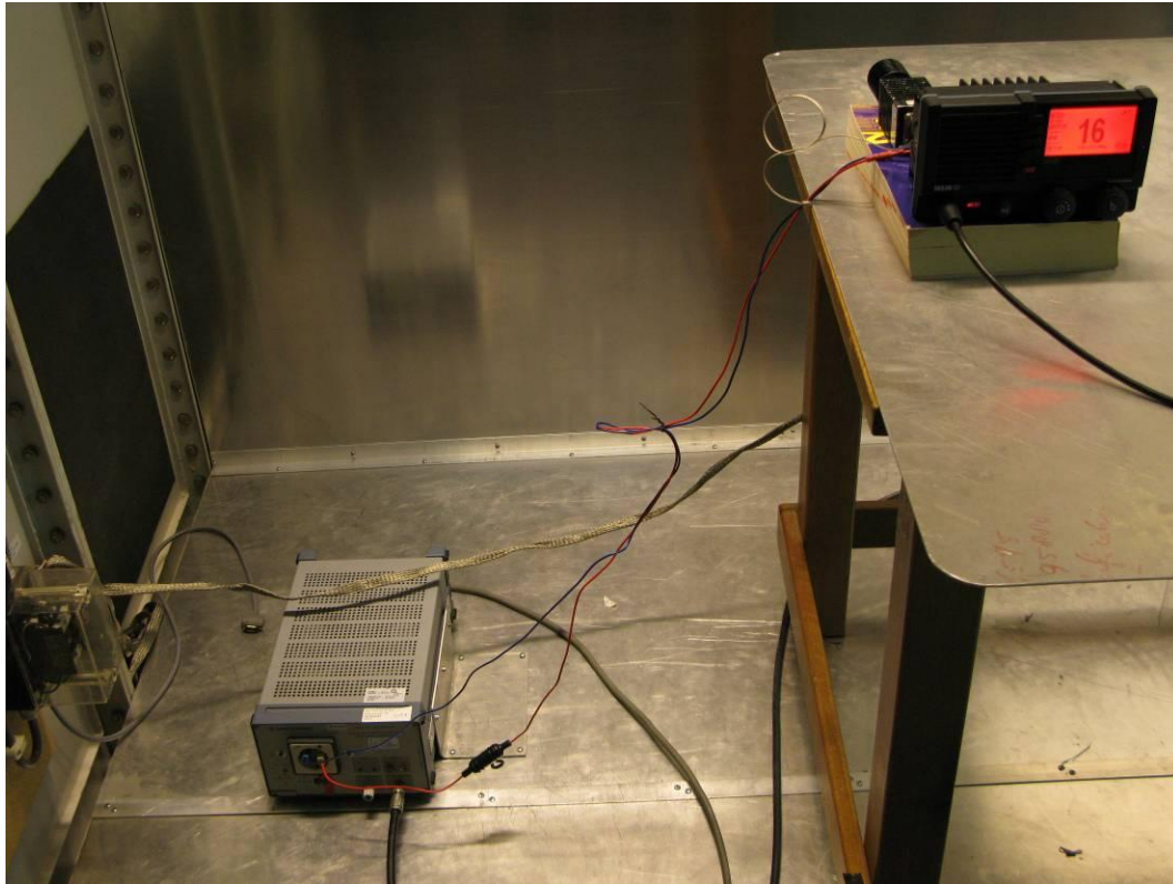
Photograph 4: - conducted emissions test
