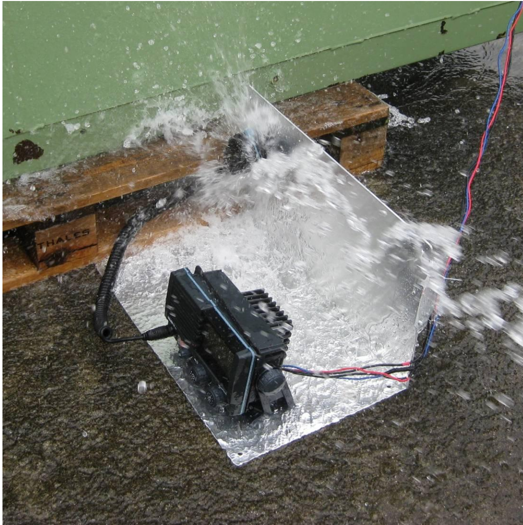
Photograph 8: - water ingress test
