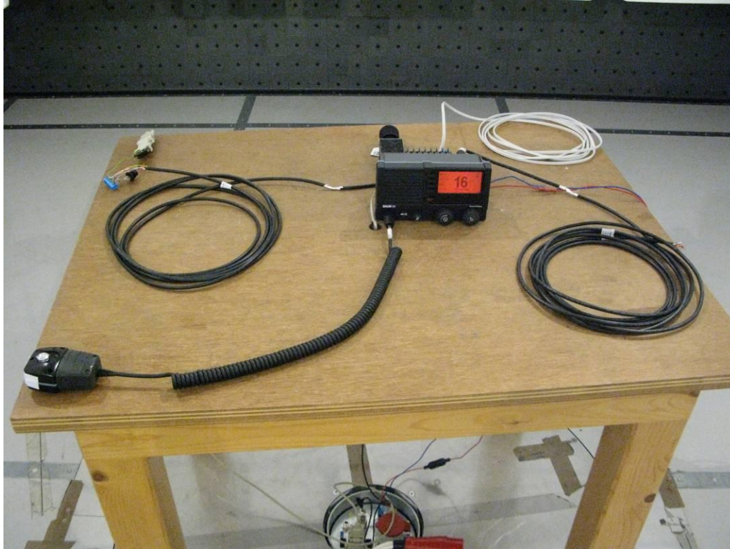
Photograph 3: - radiated emissions test, picture 3
