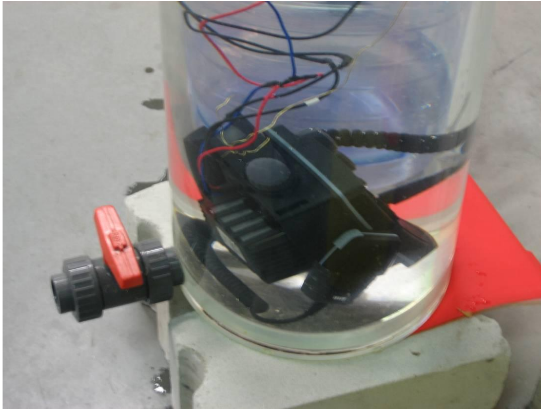
Photograph 9: - immersion test
