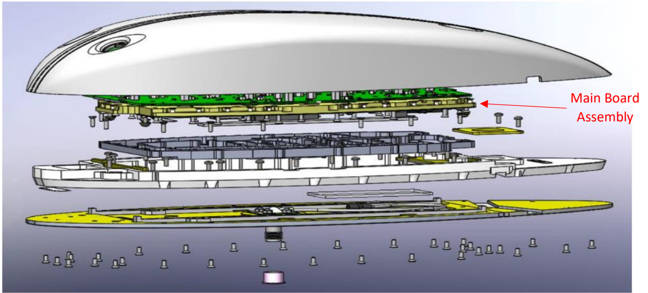
Figure 1: LGA-5005 - Mechanical View
