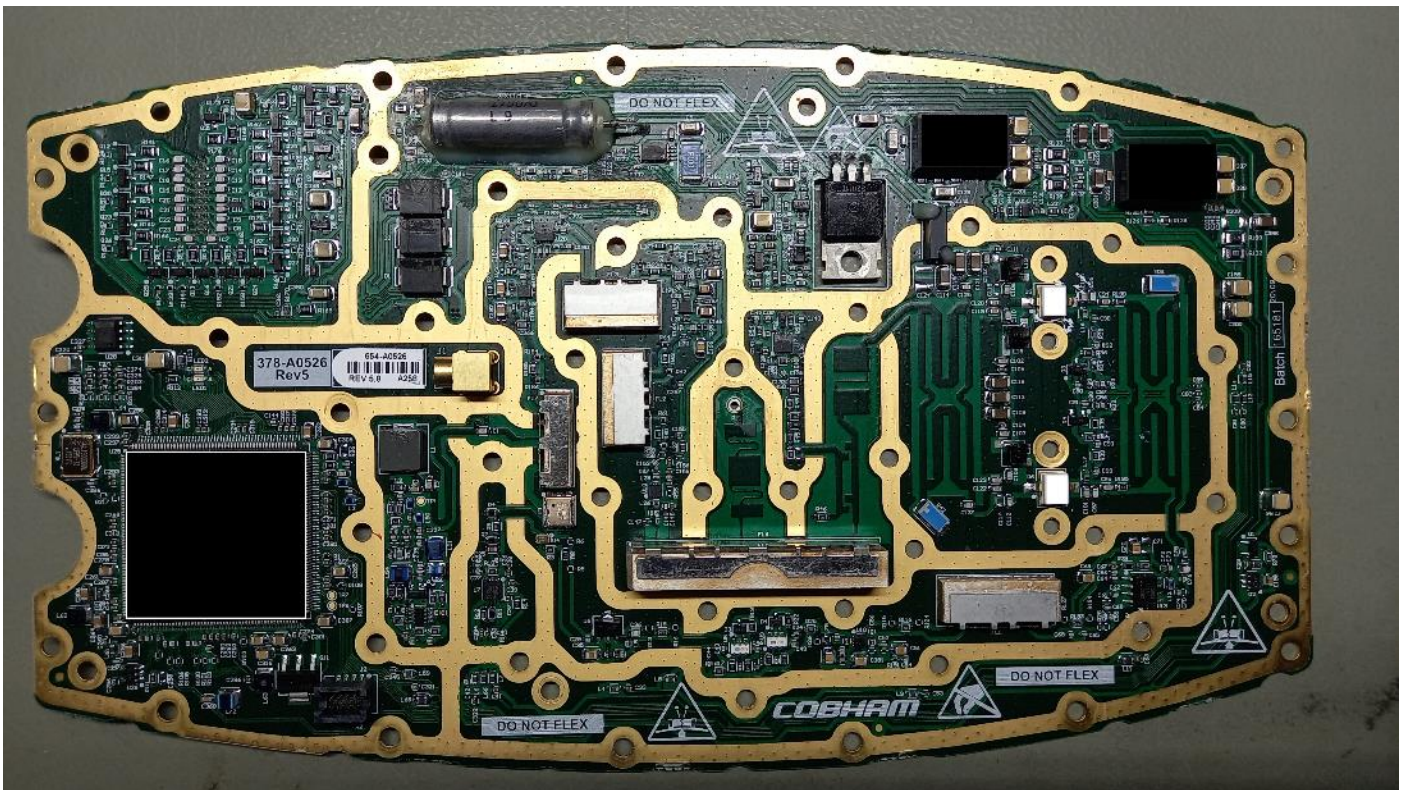
Figure 2: LGA-5005 Main Board – Top View
