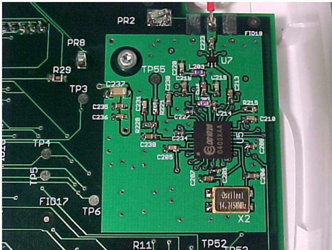
PCB Close-up of RF Section
