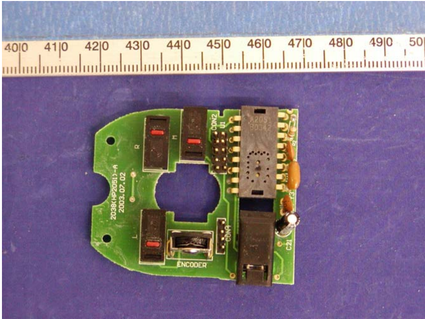
PCB 2 – Component View
