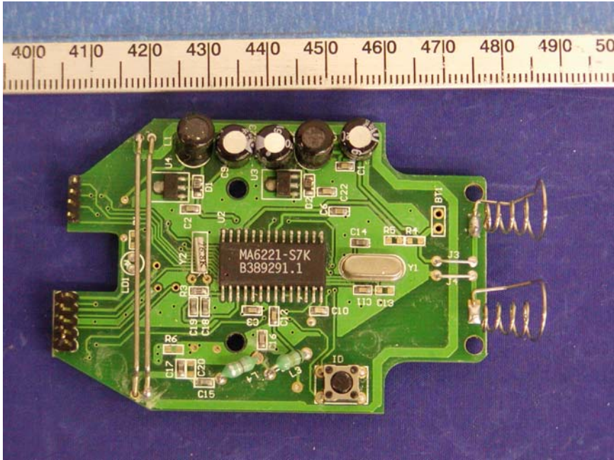
PCB 1 – Component View
