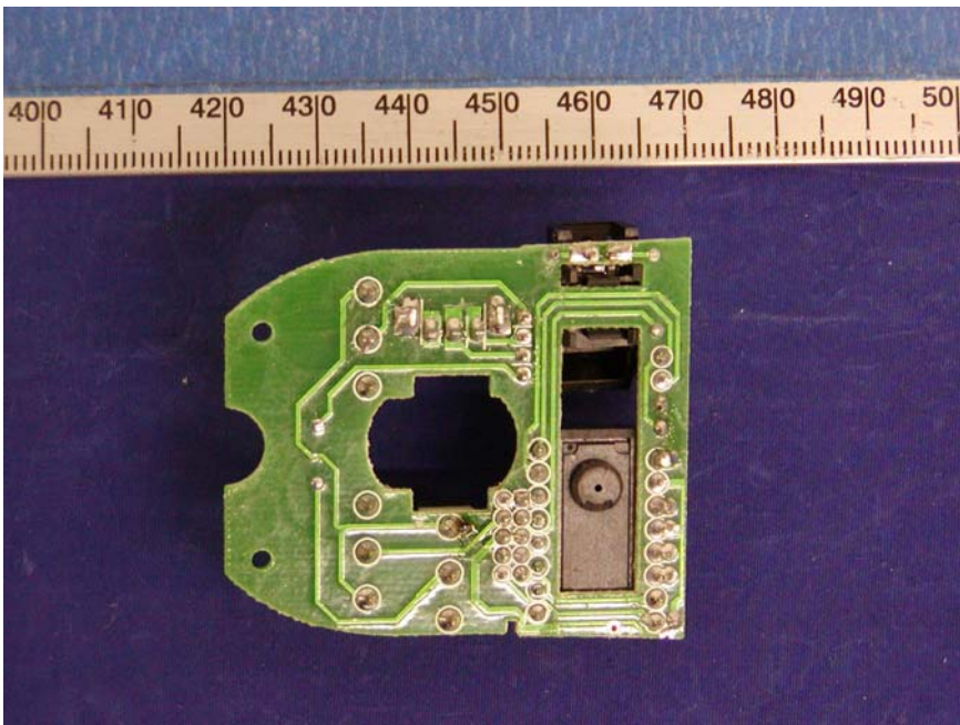
PCB 2 – Solder View
