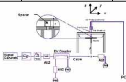
Figure 8.1 Dipole Validation Test Setup
