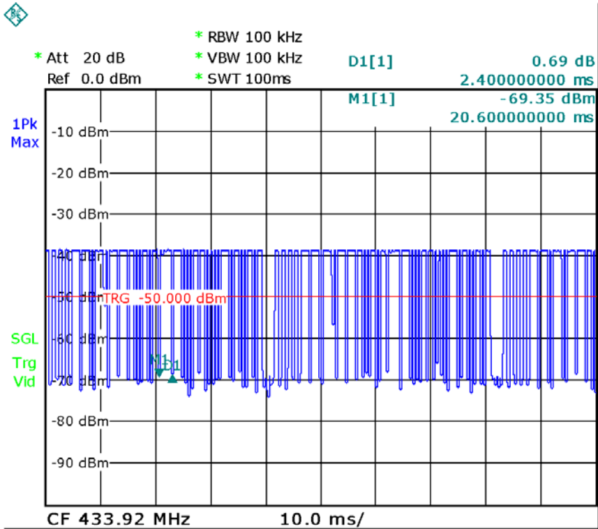
Plot 4- ON time =2.4msec
