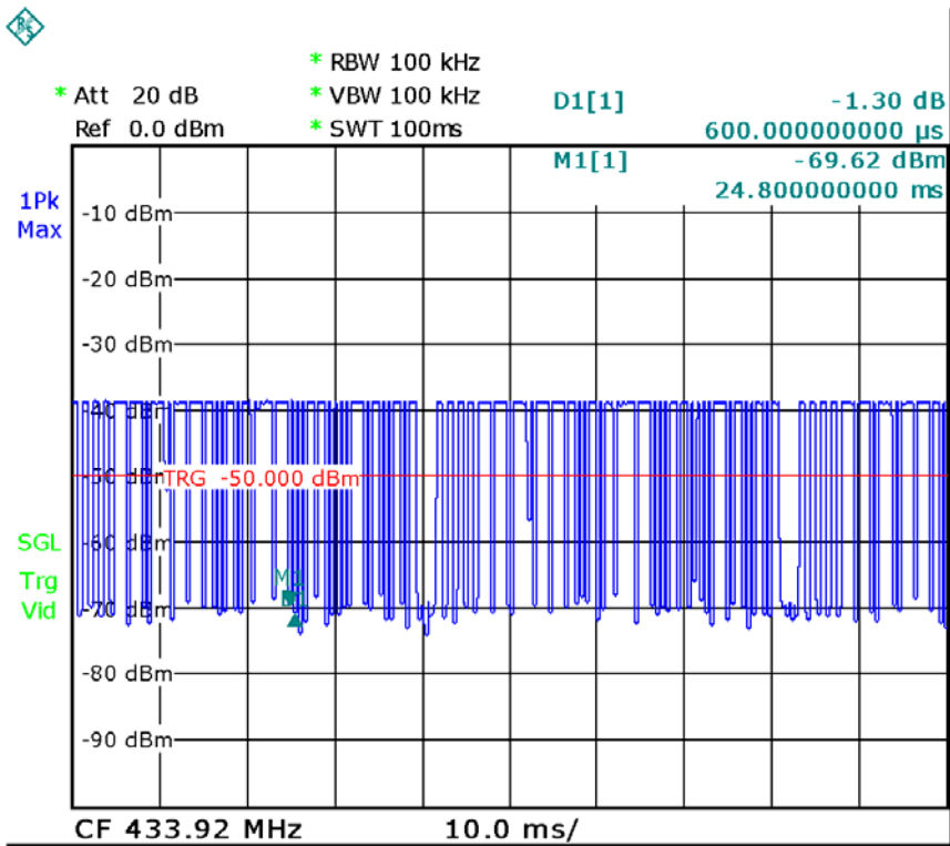
Plot 3- ON time:0.6msec
