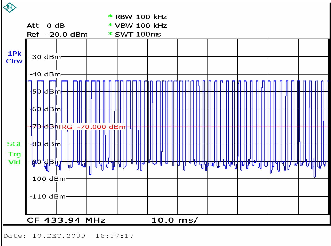
Plot 2- On Time Per 100ms(worst case)
