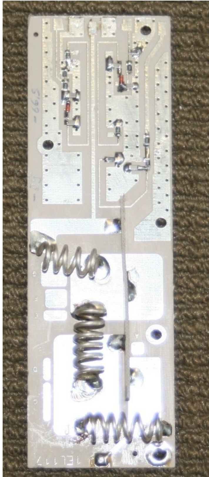
LP500 – TOP VIEW
