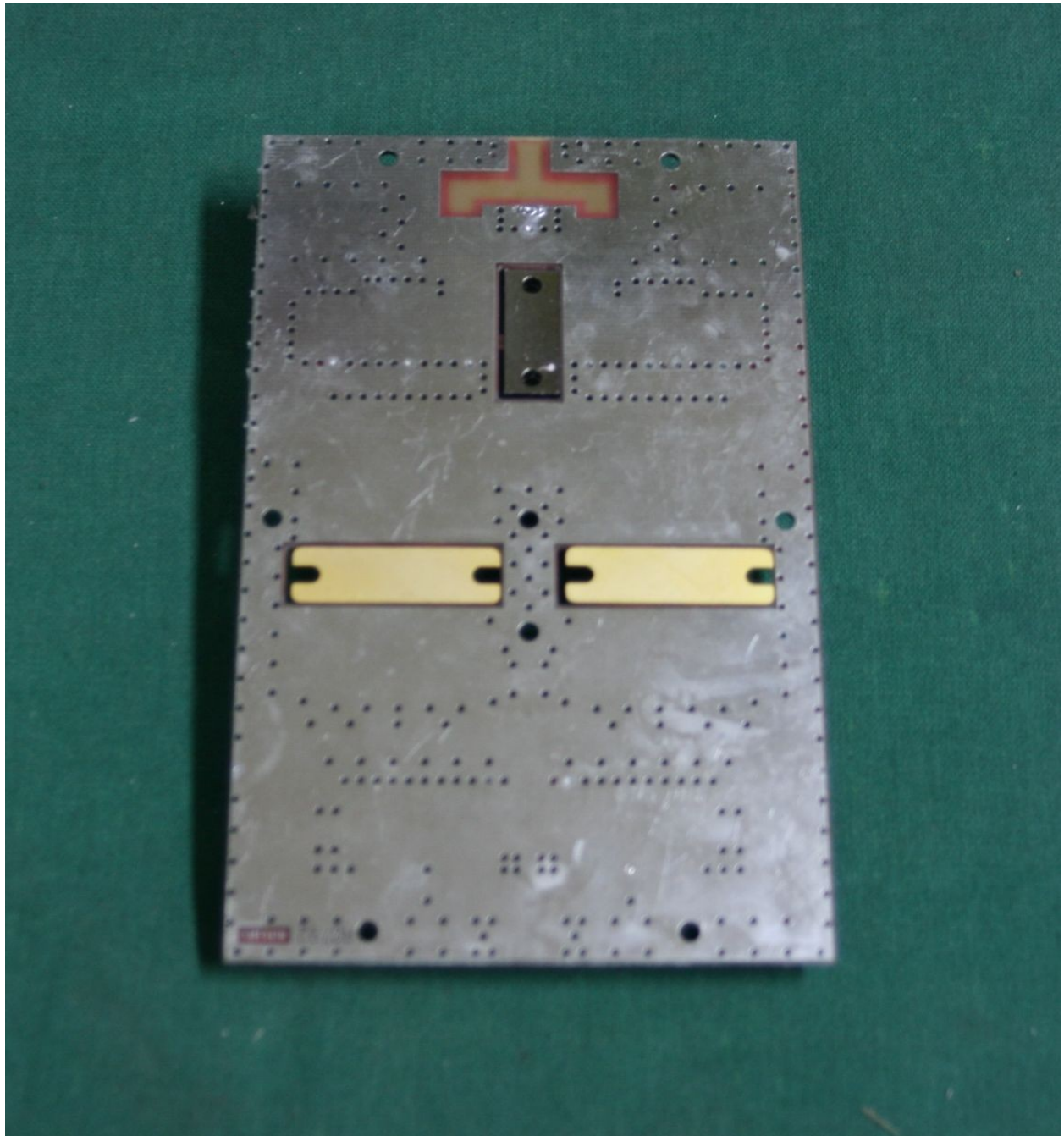
AMP 600 BOARD – REAR VIEW
