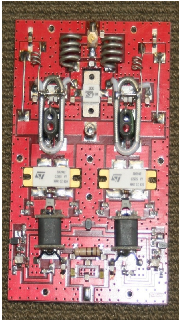
RF PALLET TOP VIEW
