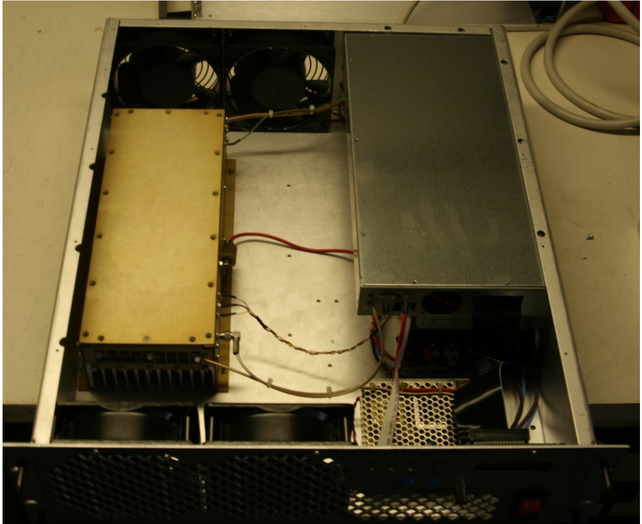
CHASSIS VIEW
