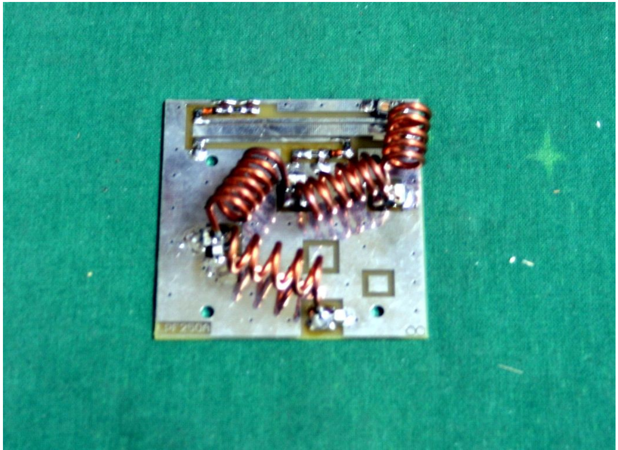
LOW PASS FILTER – FRONT VIEW
