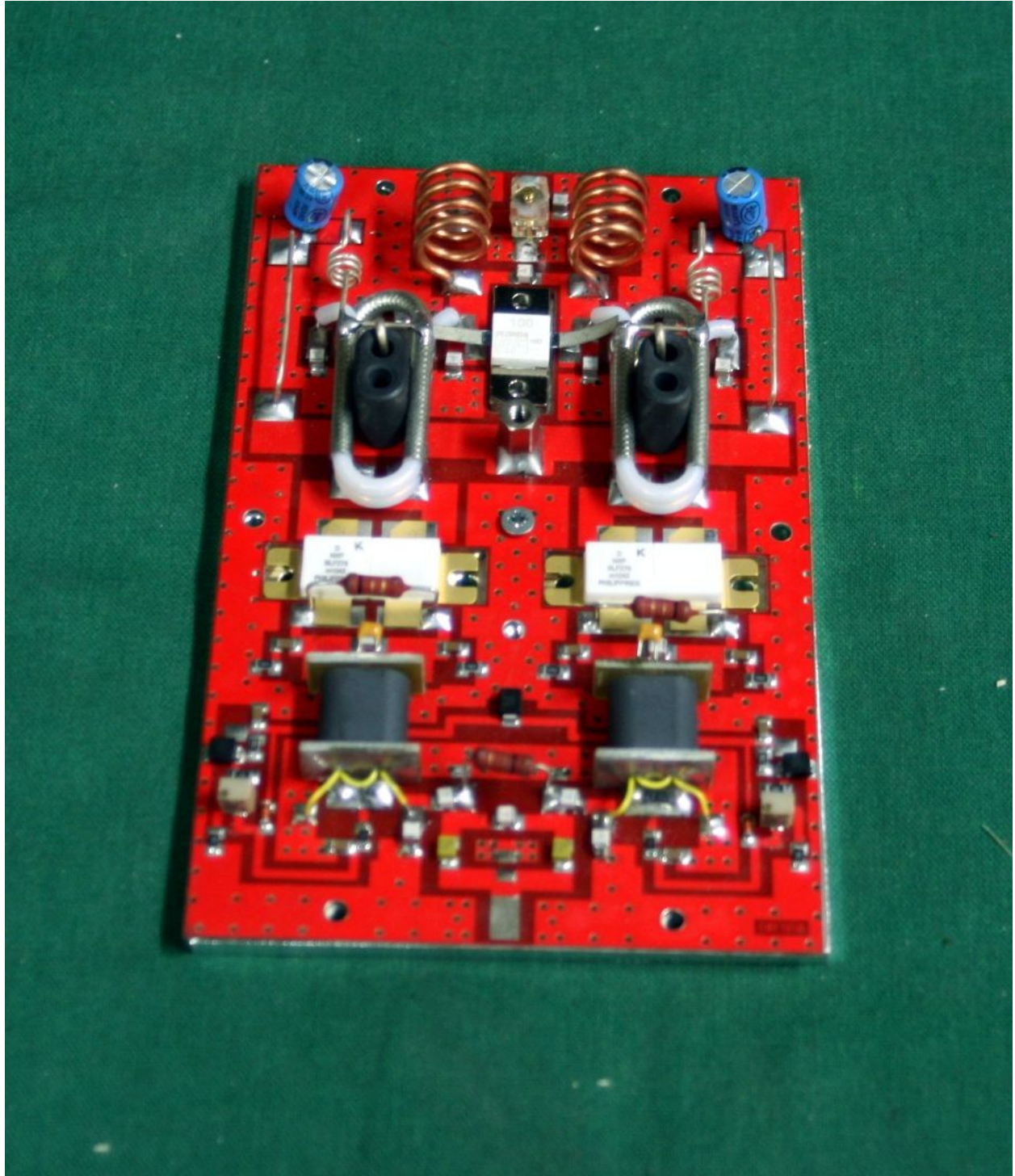
AMP 600 BOARD
