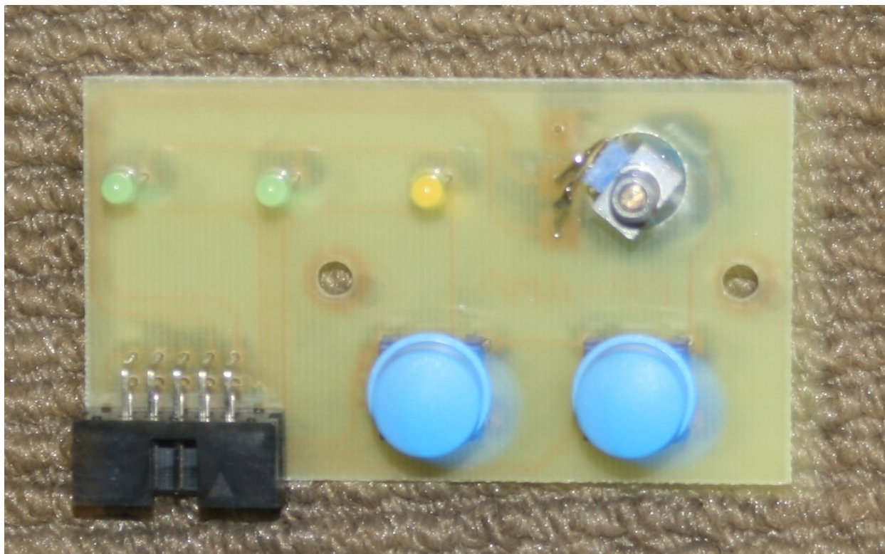
FRONT PUSH BUTTON – TOP VIEW
