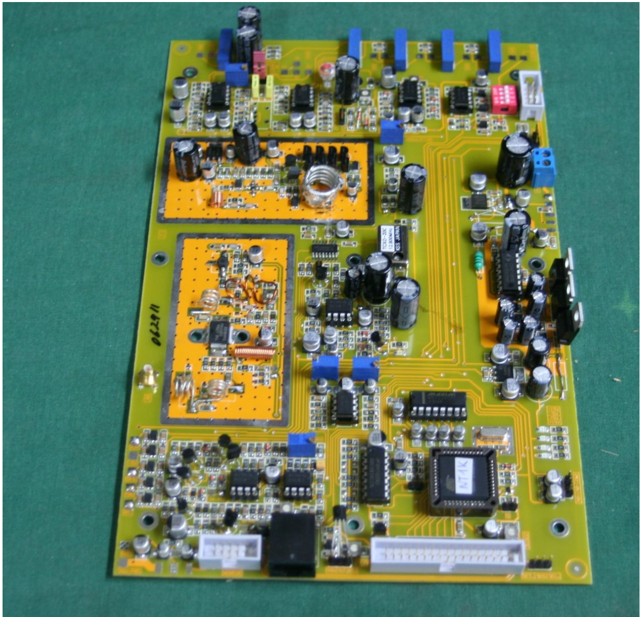
MOTHER BOARD – TOP VIEW – SHIELDS REMOVED
