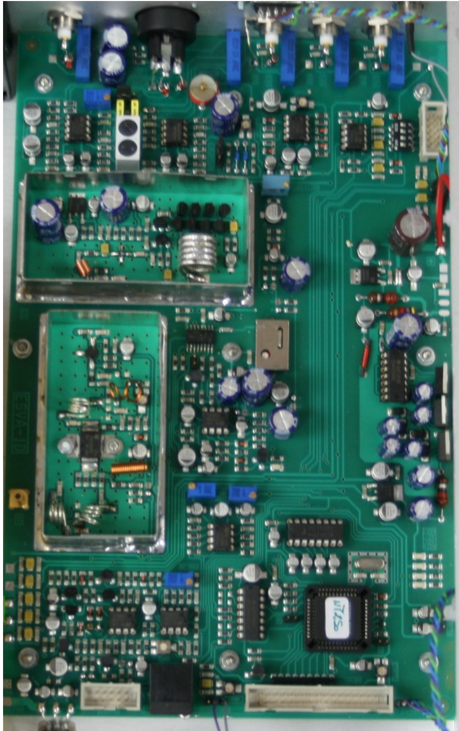
M BOARD – TOP VIEW – SHIELDS REMOVED
