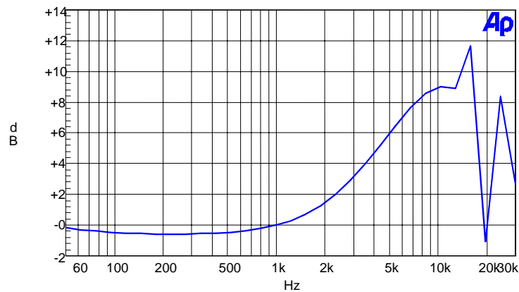
Audio Frequency Response
