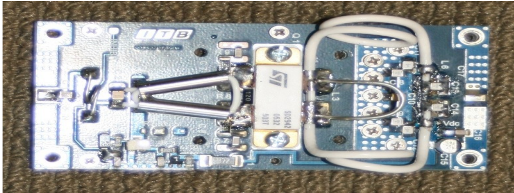
RF Pallett top view
