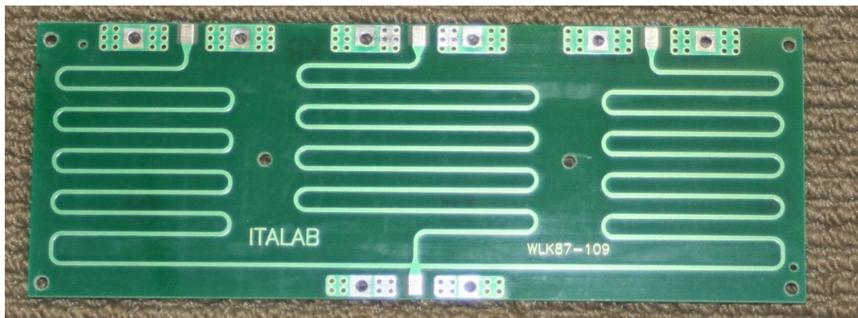
Wilk 3 LP – Top view
