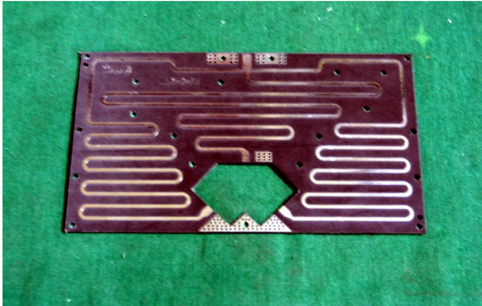
3 Way Combiner
