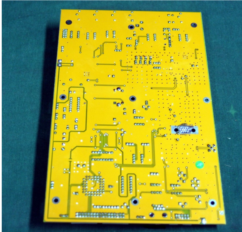
ESVA Mother Board – Rear View
