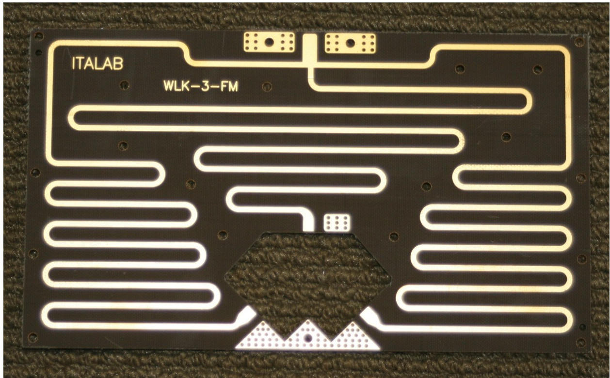
Wilk 3 HP – Top View
