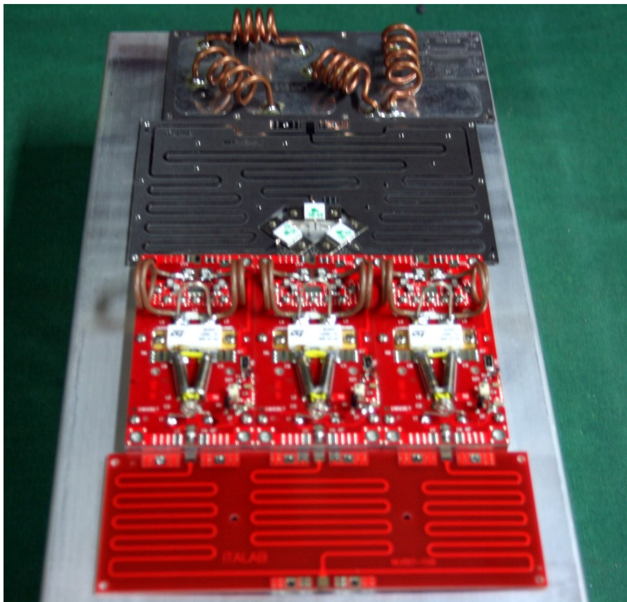
1000W RF SECTION
