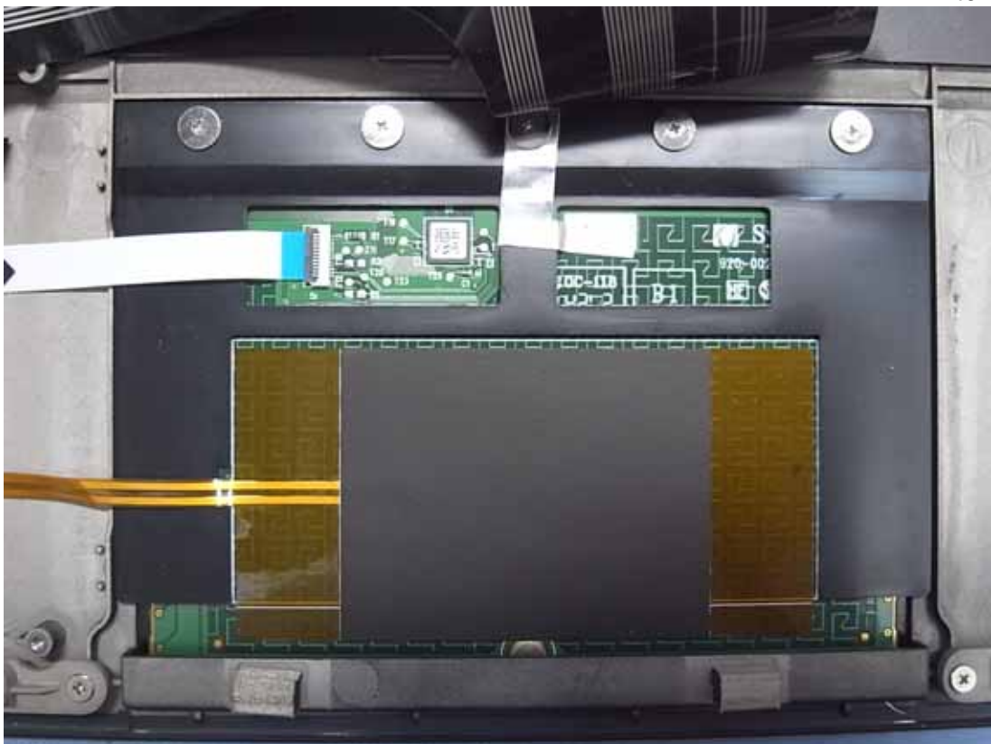
Figure 28 Internal View
