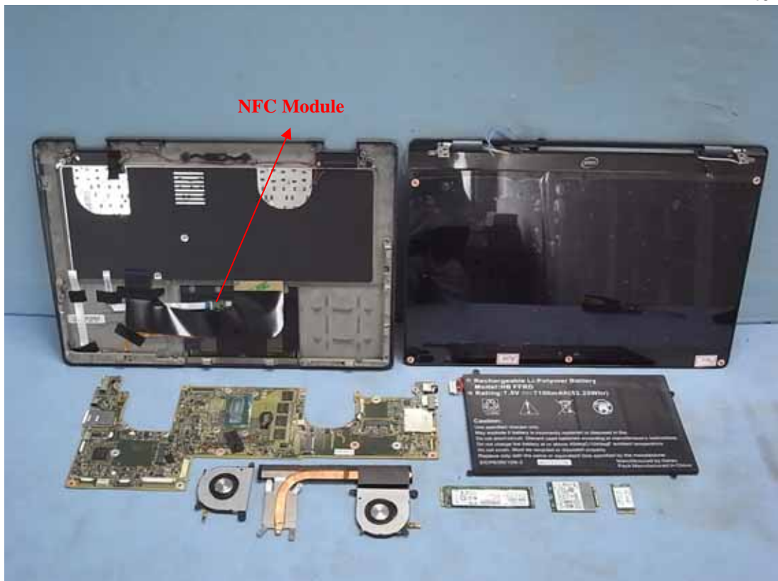
Figure 16 Internal View
