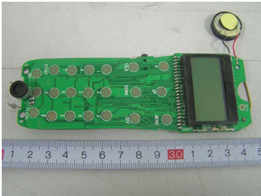
EUT- Handset PCB Front View
