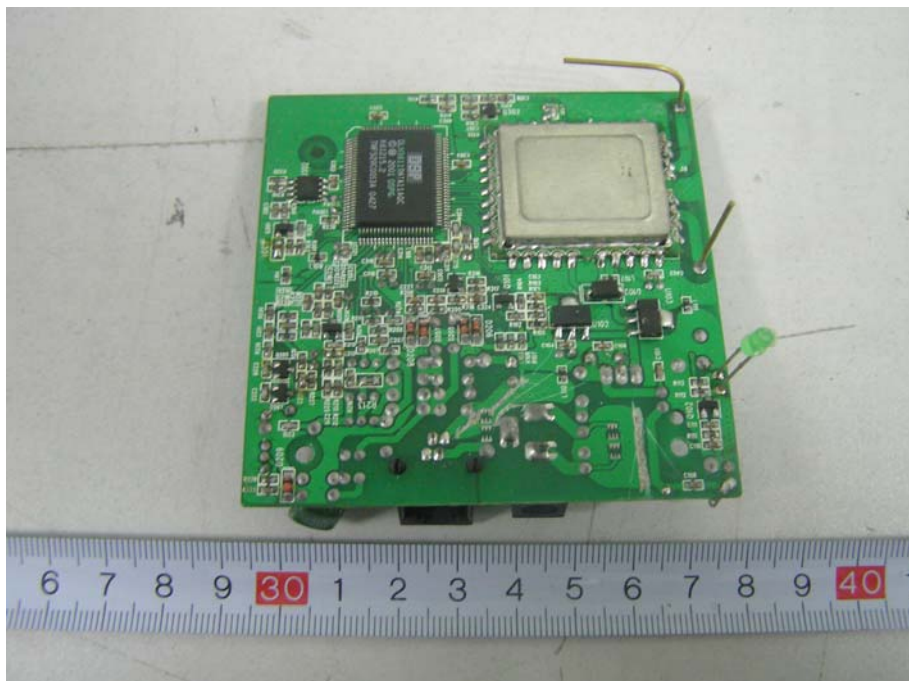
EUT- Base PCB View (2)
