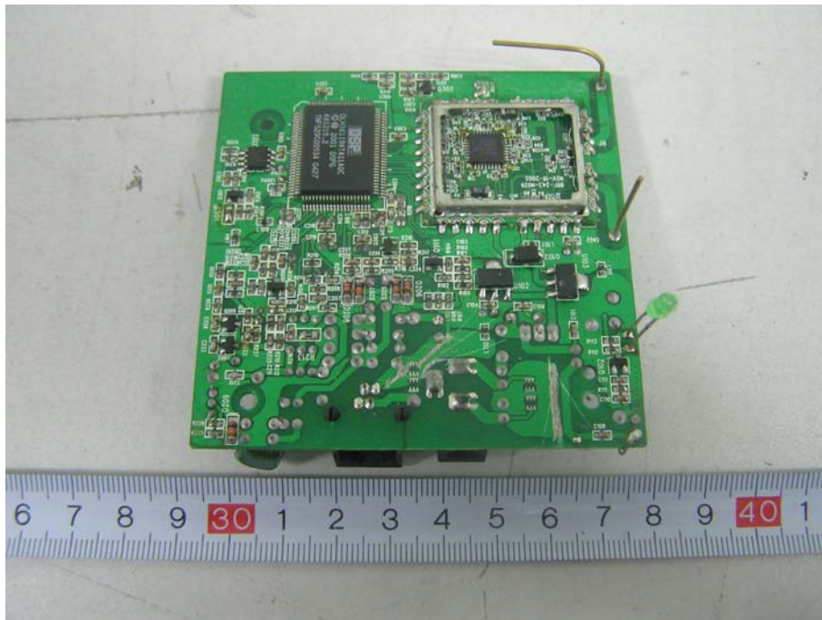
EUT- Base PCB View (3)
