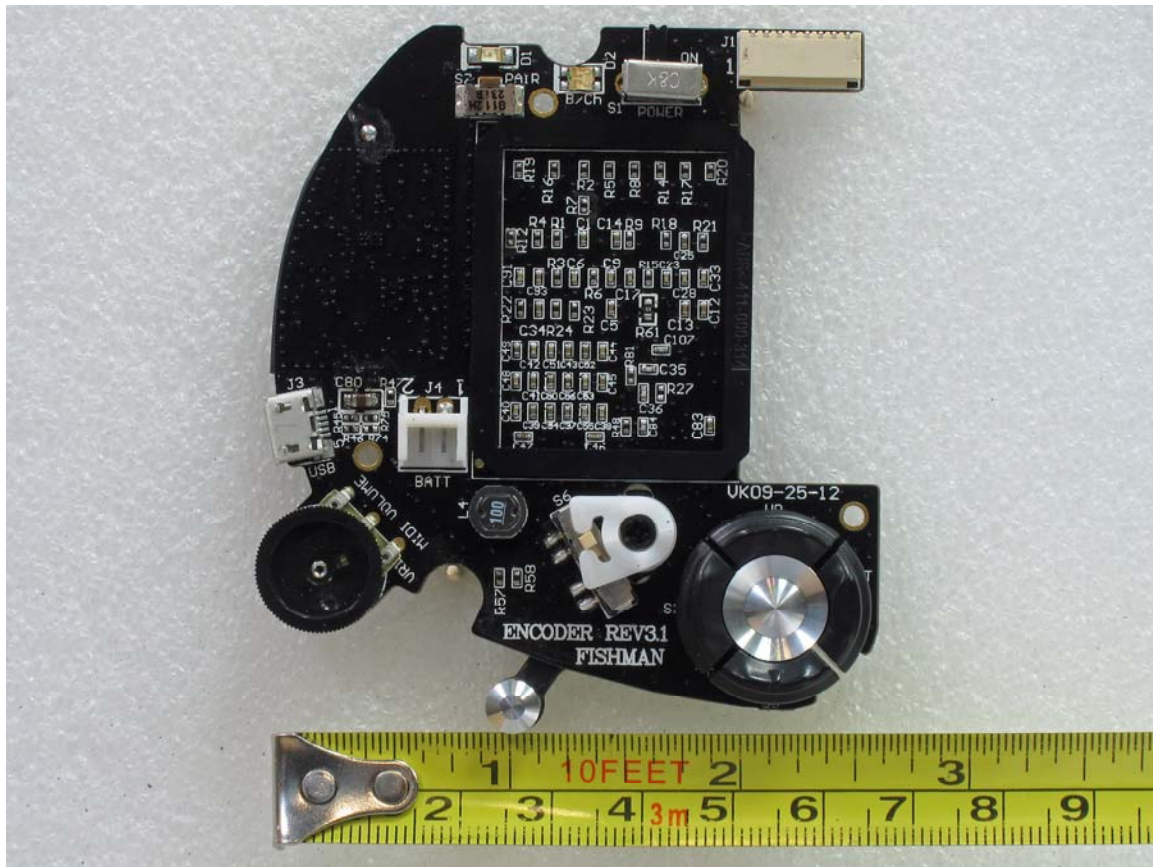
Circuit Board Front with Battery
