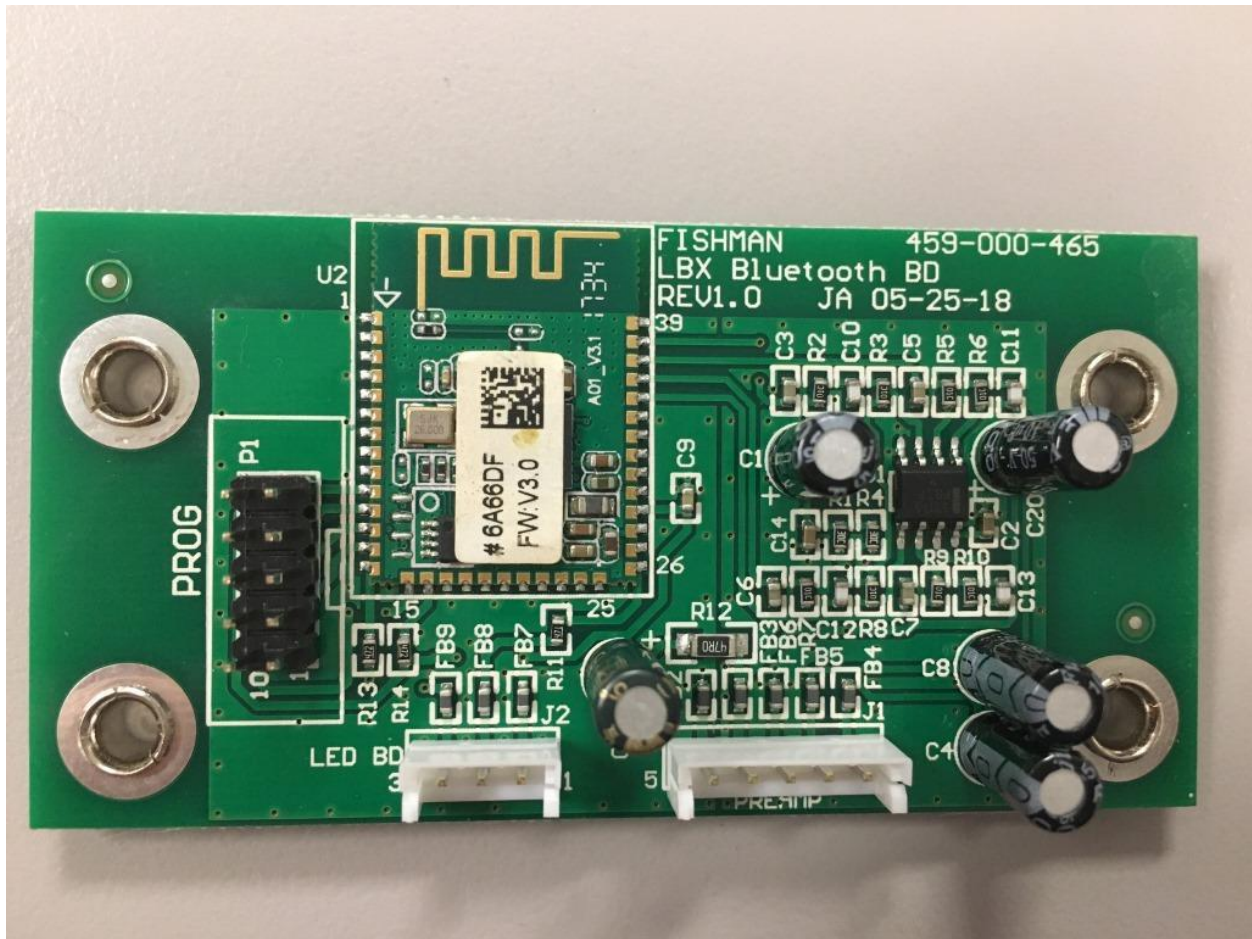
BT Mother Board Top
