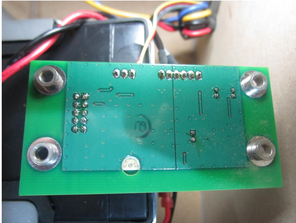
Loudbox Mini Charge, Bluetooth Board Close-up, Bottom View
