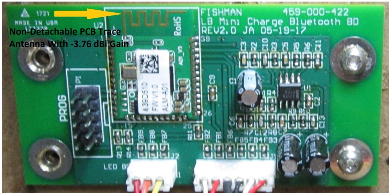
Loudbox Mini Charge, Bluetooth Board Close-up, PCB Trace Antenna -3.76 dBi Gain
