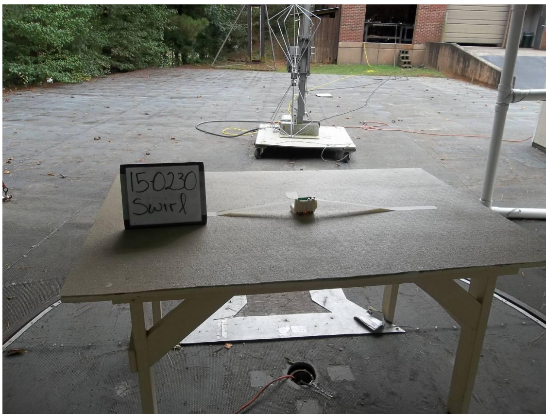
Figure 3. Radiated Emissions Test Configuration, 30-200 MHz
