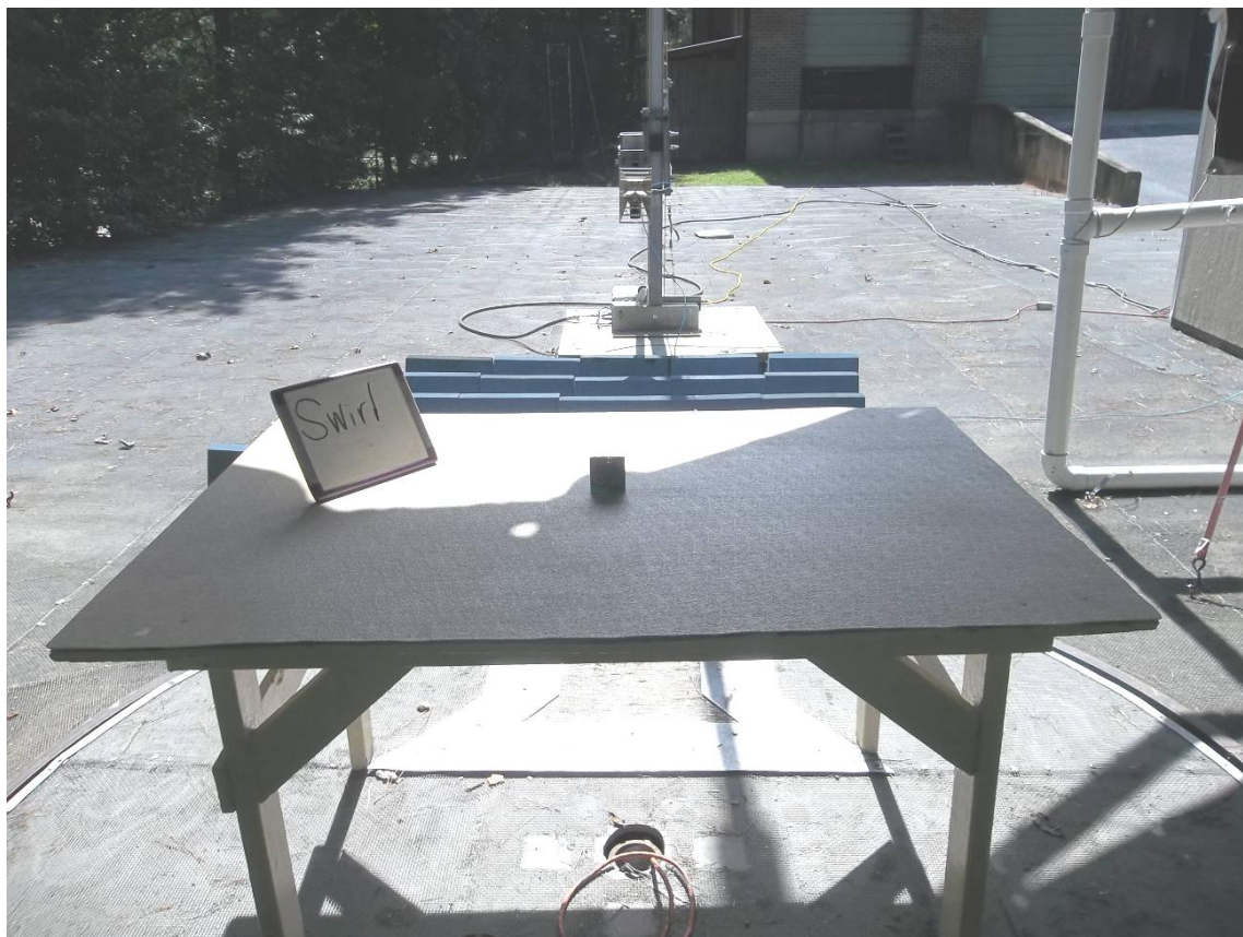
Figure 5. Radiated Emissions Test Configuration, above 1 GHz
