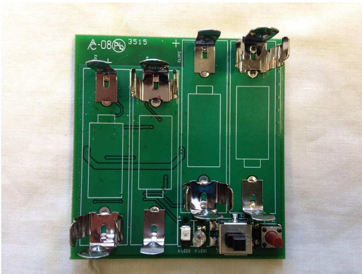
Figure 3. Batteries Removed
