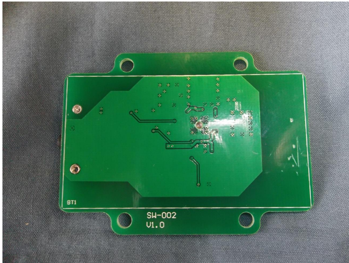
Figure 4. Solder Side (Battery Holder Removed)
