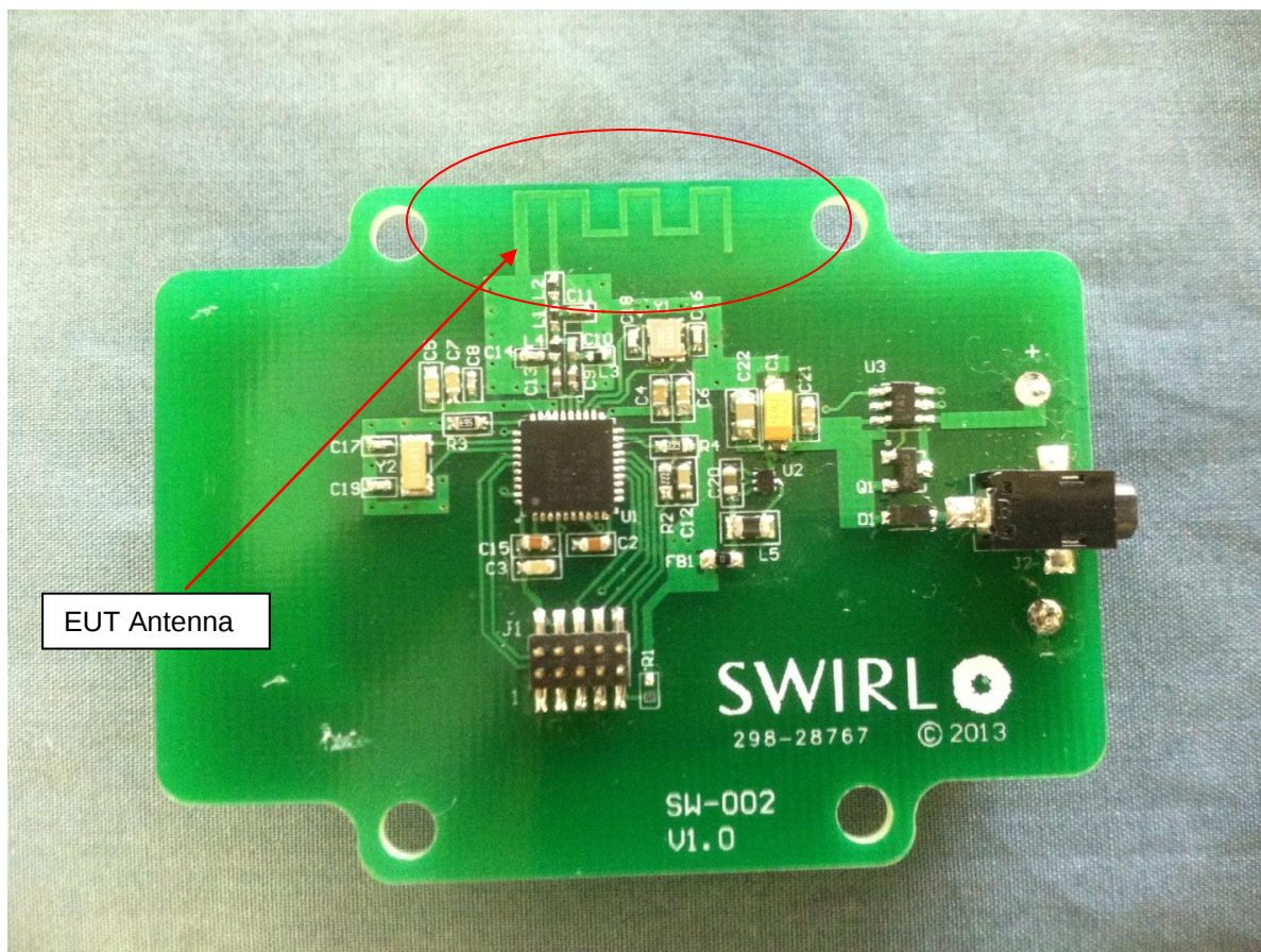
Figure 3. Component Side
