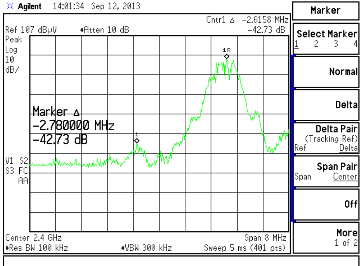
Figure 9. Radiated Band Edge – Low Channel Delta
