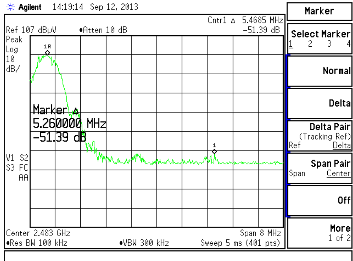
Figure 7. Radiated Band Edge – High Channel Delta
