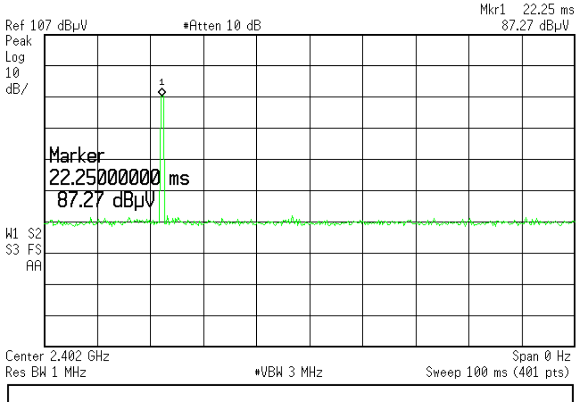
Figure 3. Transmitter Pulse Width (100ms)
