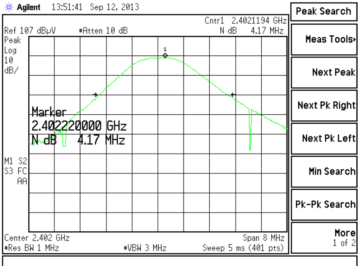
Figure 4. Low Ch Bandwidth
