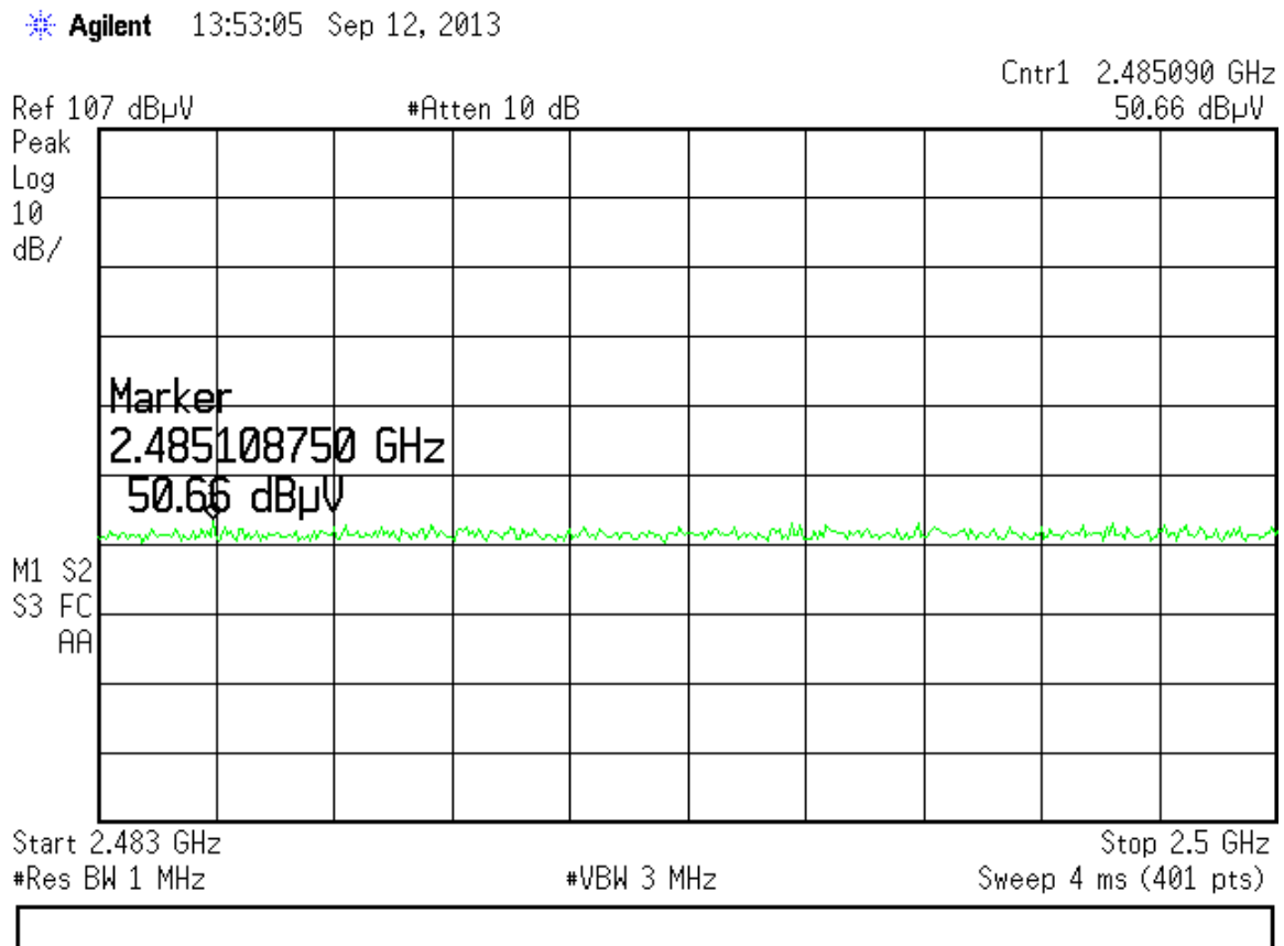
Figure 8. Emissions within the band 2.483-2.5 GHz
