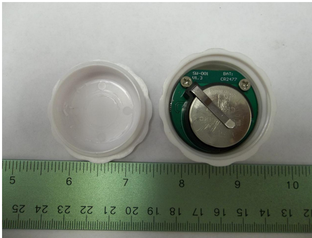
Figure 1. Enclosure Open
