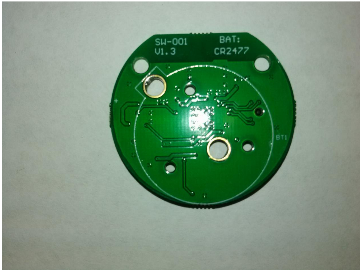
Figure 4. Solder Side (Battery Holder Removed)
