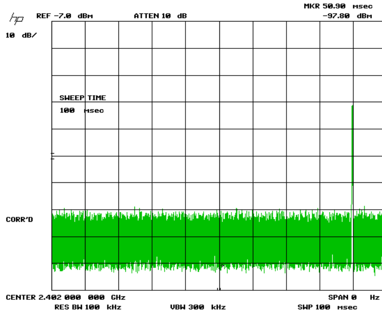
Figure 3. Transmitter Pulse Width (100ms)
