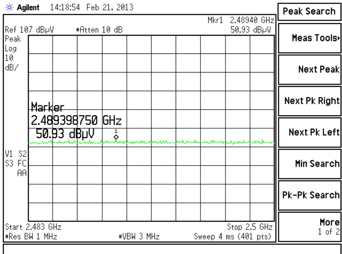
Figure 8. Emissions within the band 2.483-2.5 GHz
