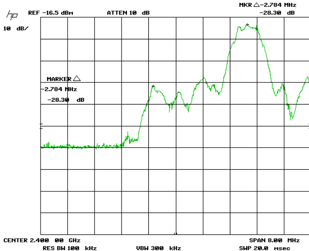
Figure 9. Radiated Band Edge – Low Channel Delta
