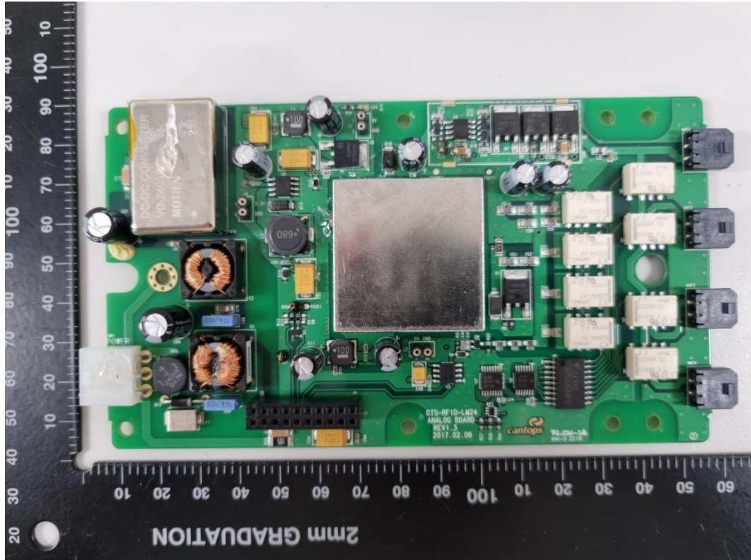
Main Board(Power & Anetnna, Front)
