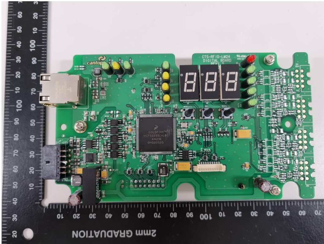
Main Board(System, Front)
