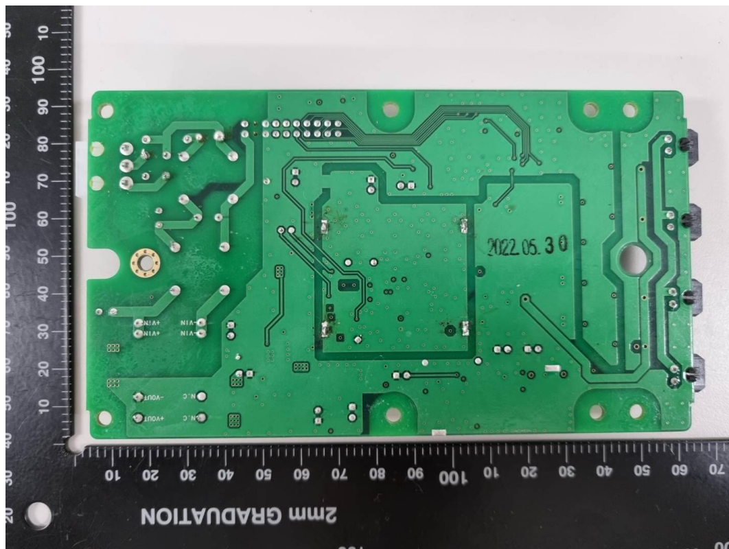
Main Board (Power & Anetnna ,Rear)
