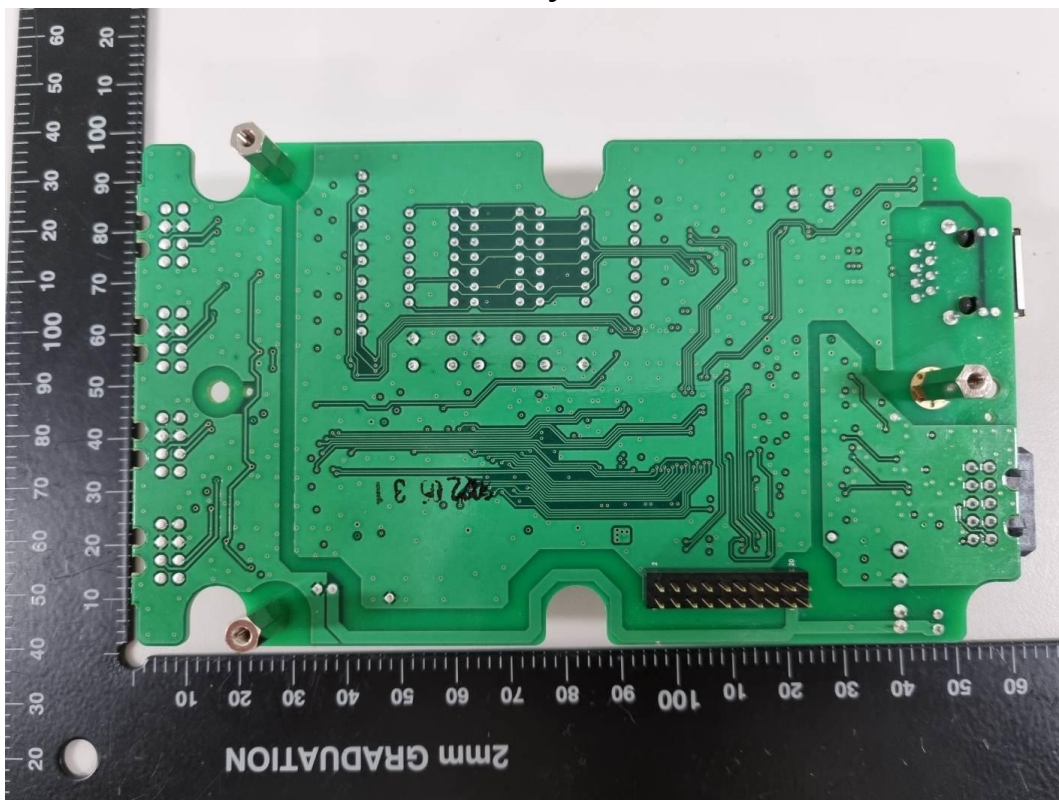
Main Board (System ,Rear)
