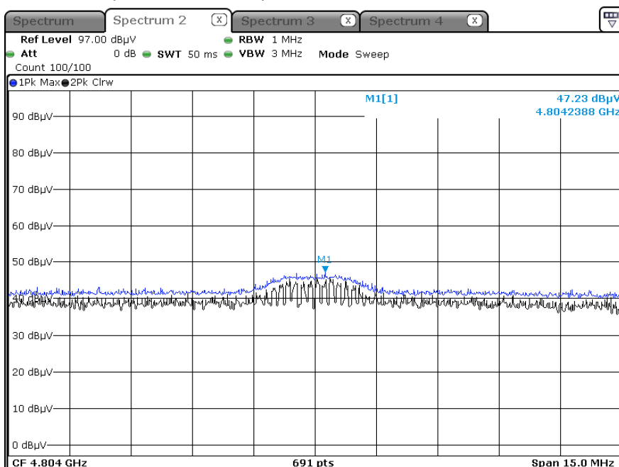
Radiated Spurious Emissions plot – Peak Result (Ch.0 2nd Harmonic, Y-V)
