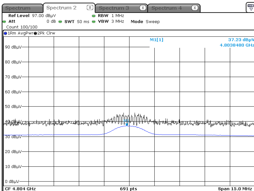
Radiated Spurious Emissions plot – Average Result (Ch.0 2nd Harmonic, Y-V)
