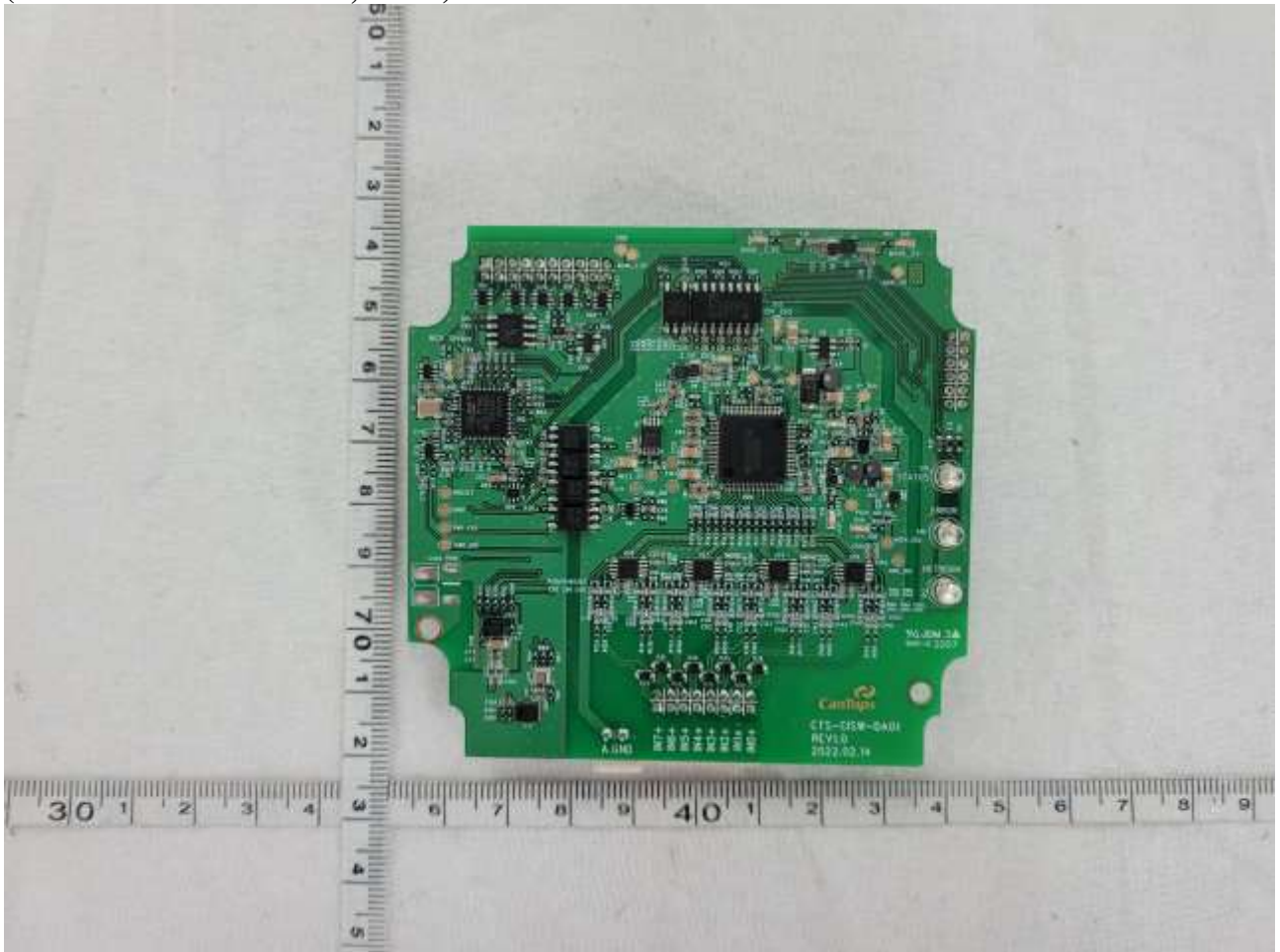
(CTS-CISW-DA01 Board, Front)
