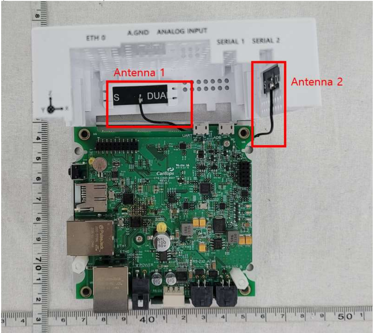
(Internal Photo - Antenna)
