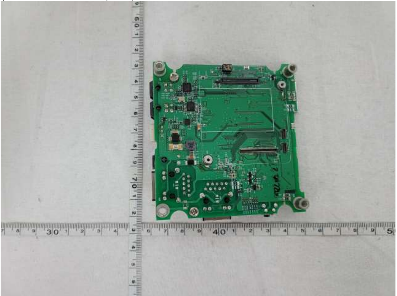
(CTS-CISW-BS01 Board, Back)
