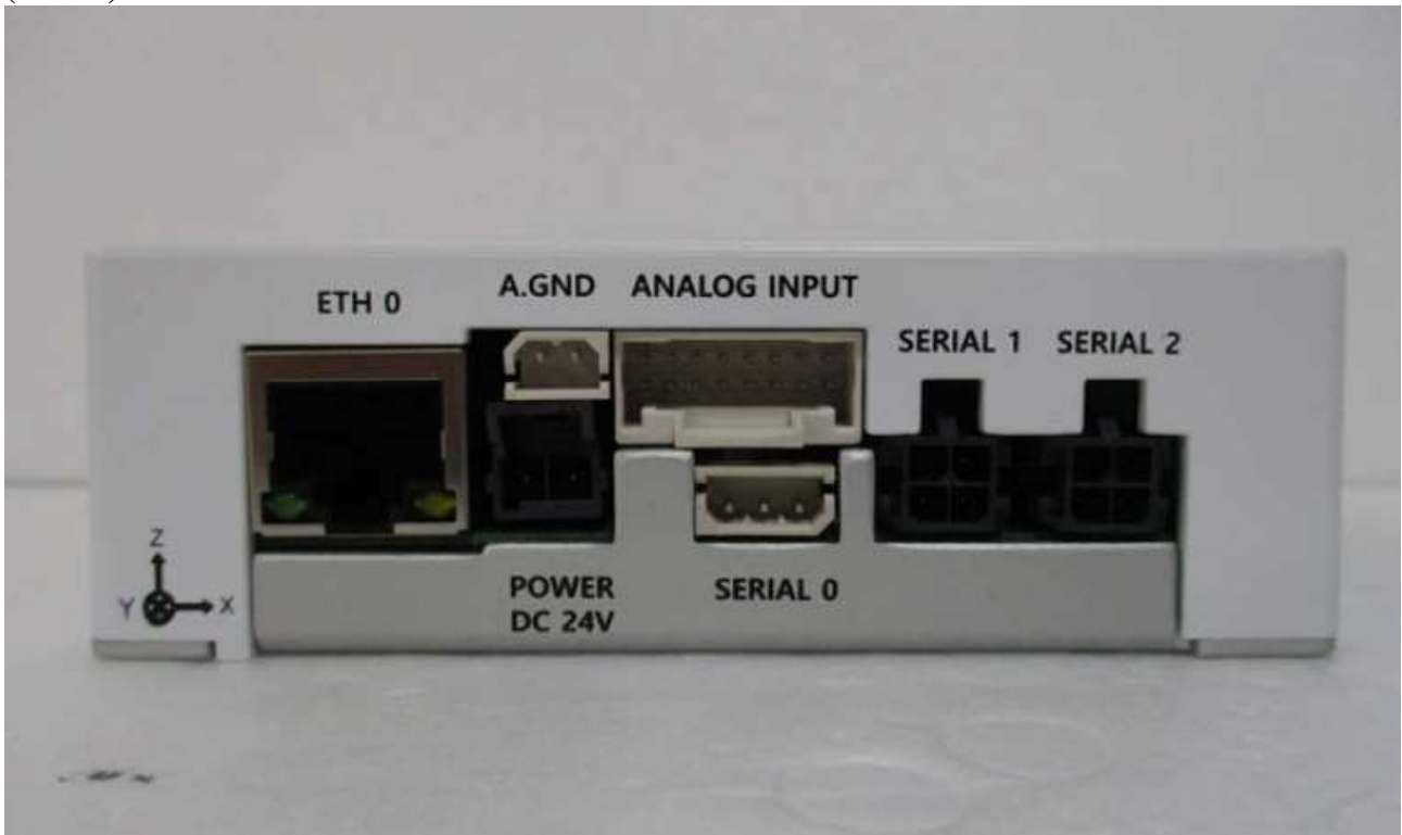
(Port 2)
