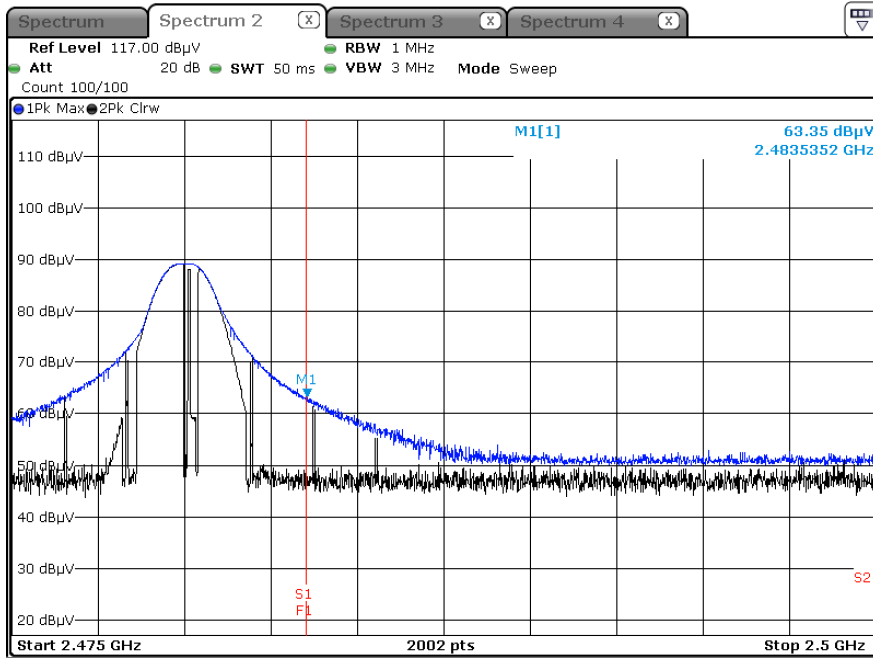
Radiated Restricted Band Edges plot – Average & Peak ( \pi/4 DQPSK, Ch.78, X-V)
