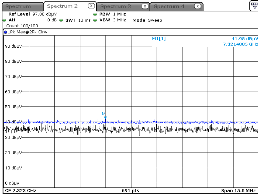
Radiated Spurious Emissions plot – Average & Peak (GFSK, Ch.39 3rd Harmonic, X-V)
