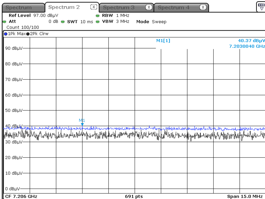
Radiated Spurious Emissions plot – Average & Peak ( \pi/4 QPSK, Ch.0 3rd Harmonic, X-V)
