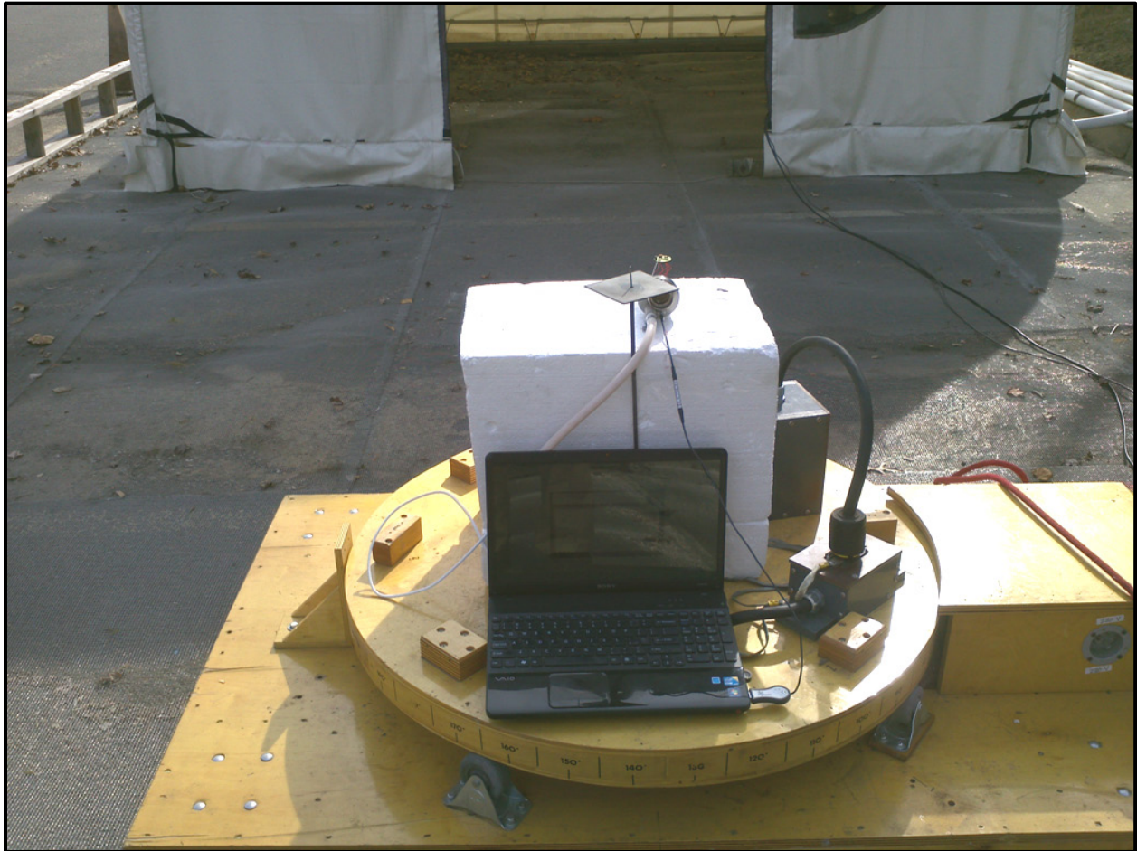
Photograph 4: Radiated Testing – Field Strength Measurement
