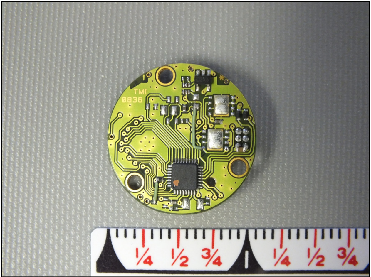
Photograph 7: Top View
