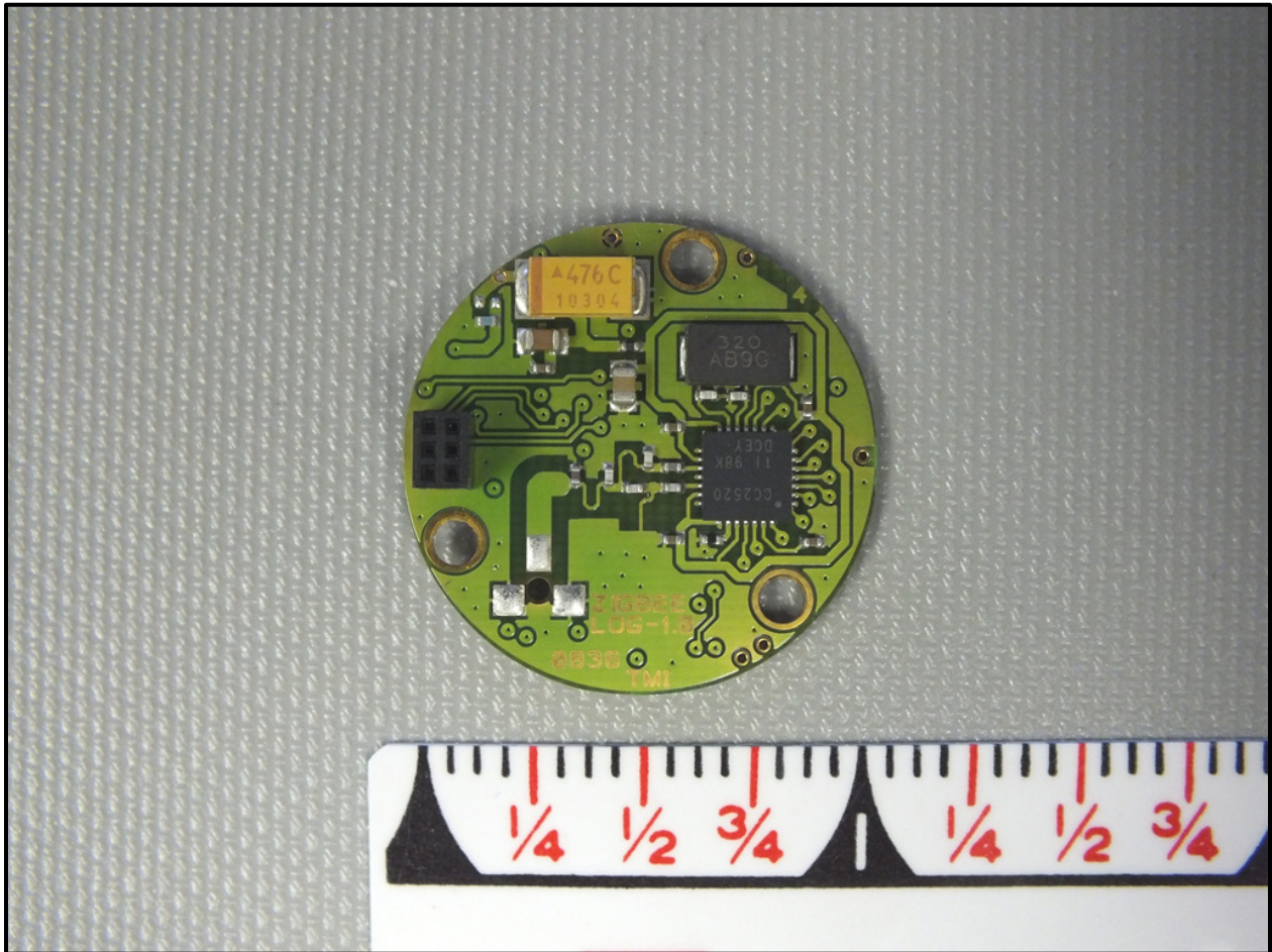
Photograph 8: Bottom View
