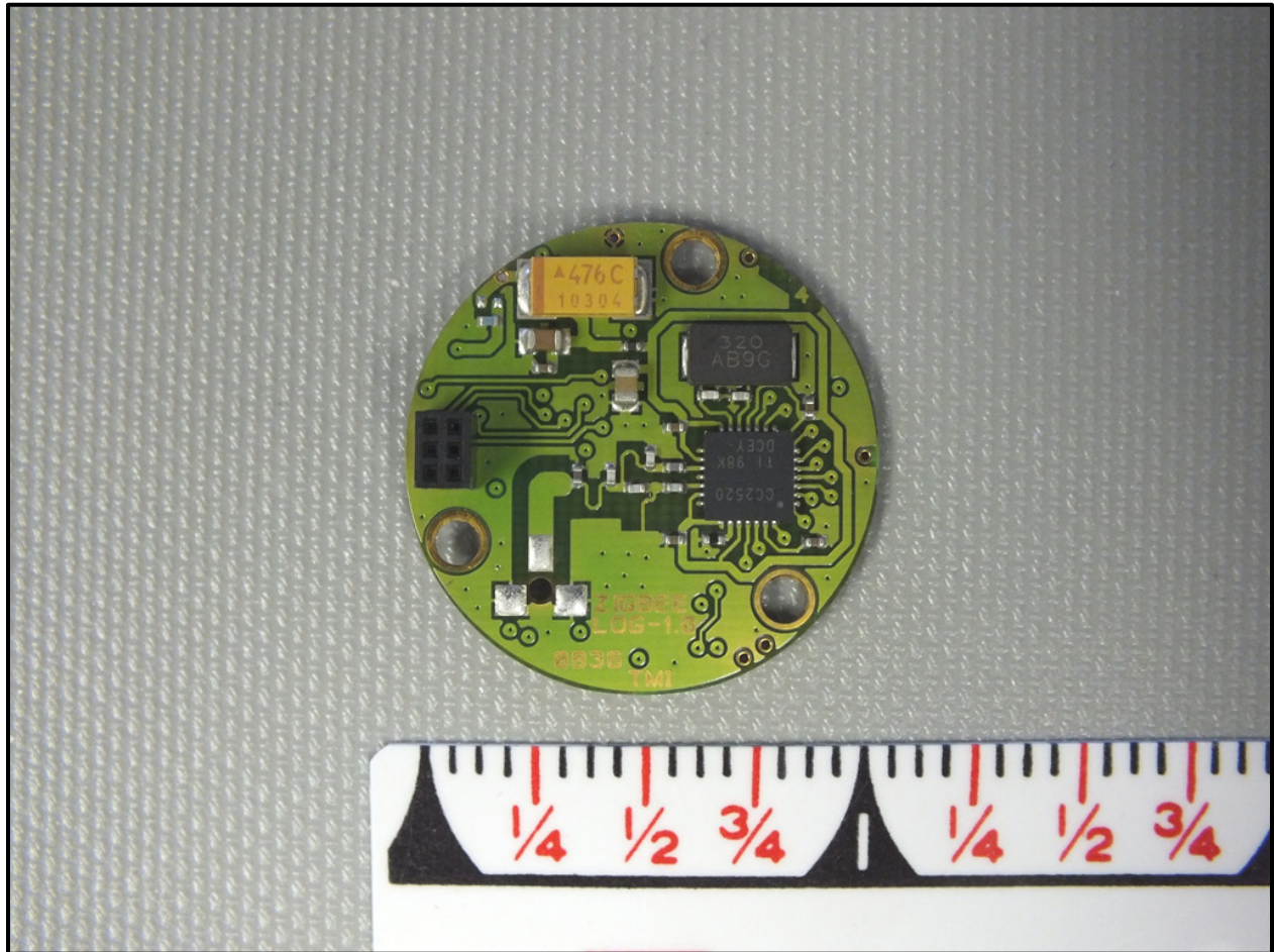
Photograph 6: Bottom View
