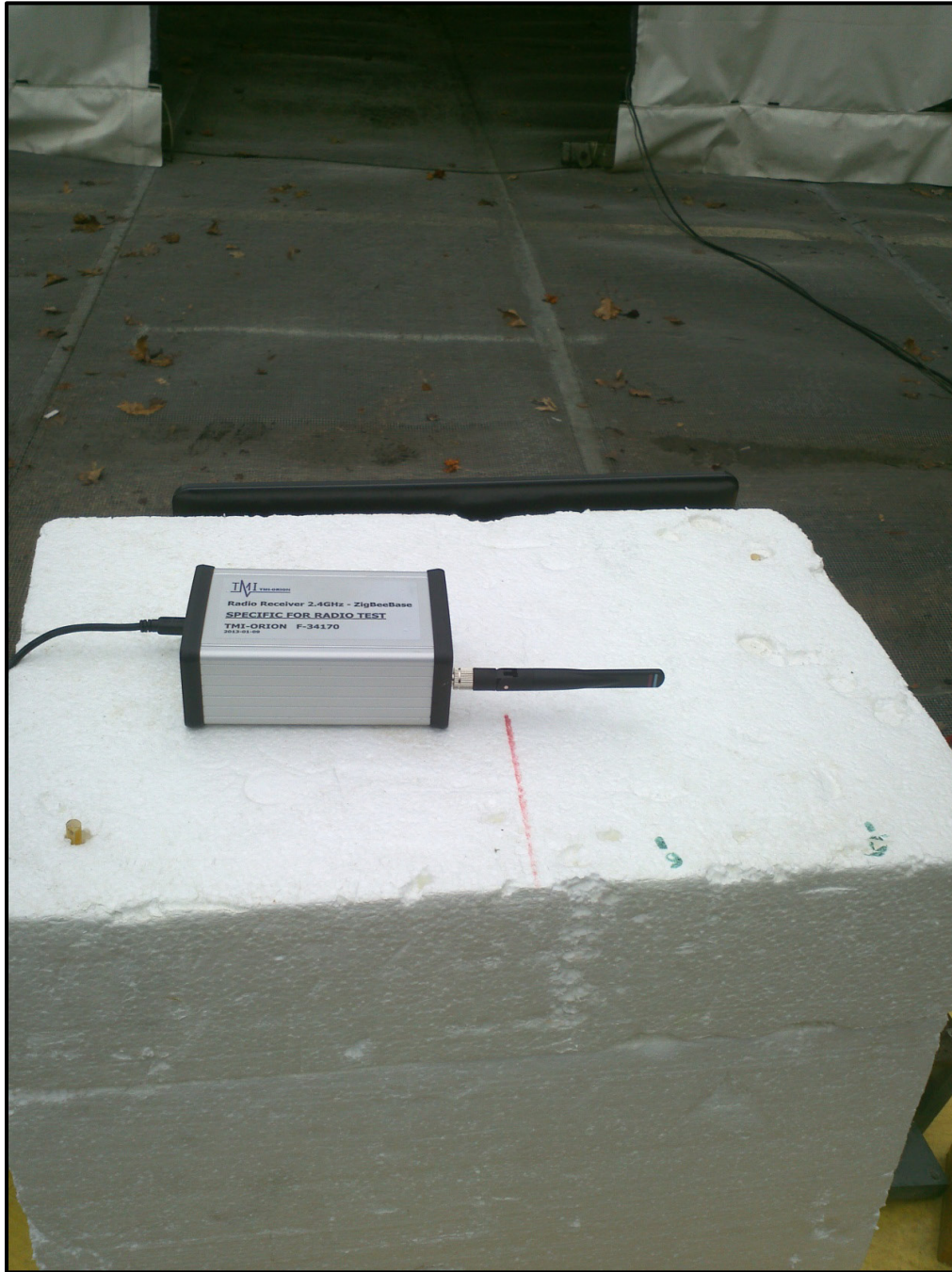
Photograph 2: Radiated Testing – Rear View
