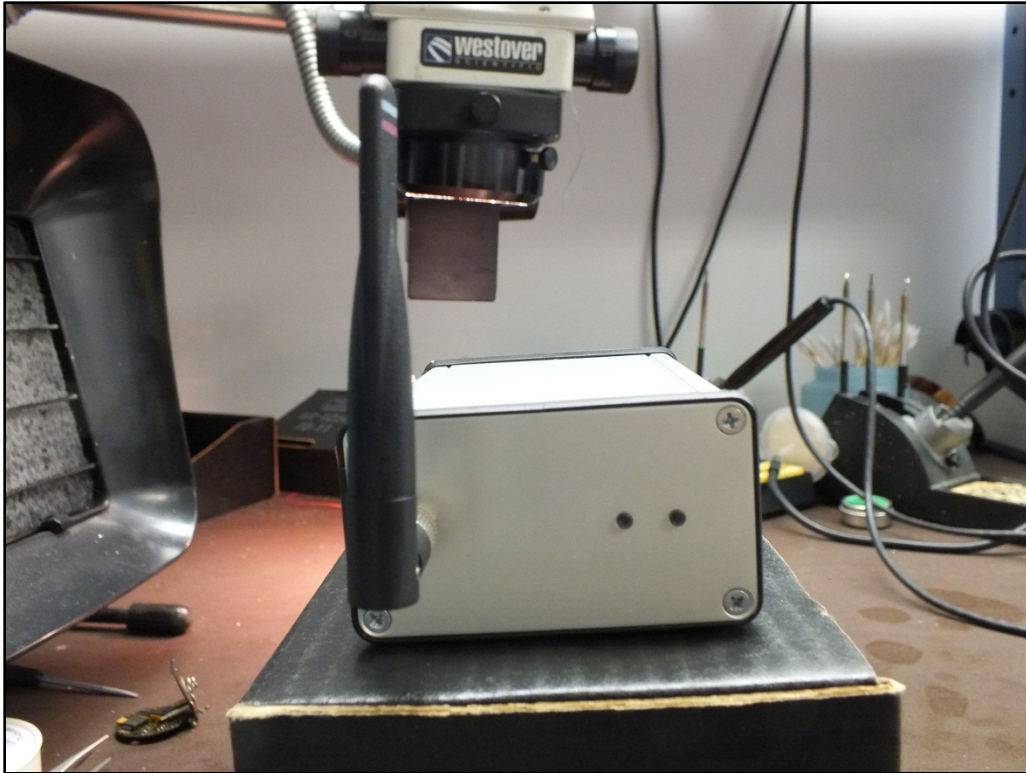
Figure 4: Radio Receiver Rear View
