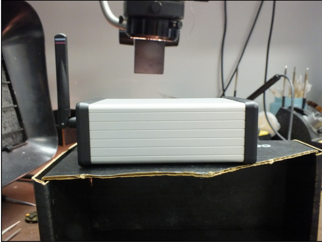
Figure 2: Radio Receiver Side View
