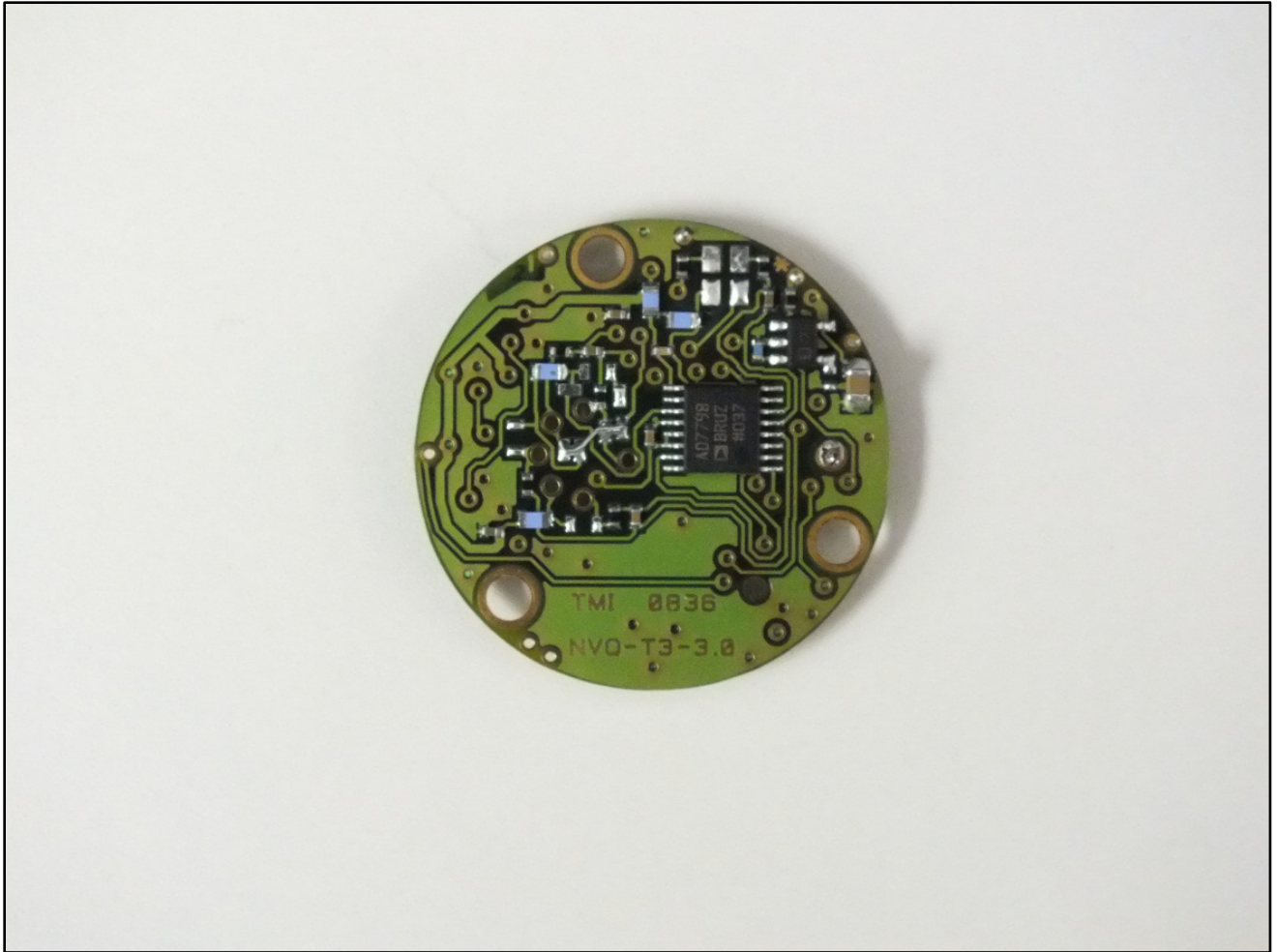
Figure 1: Memory Board Top View
