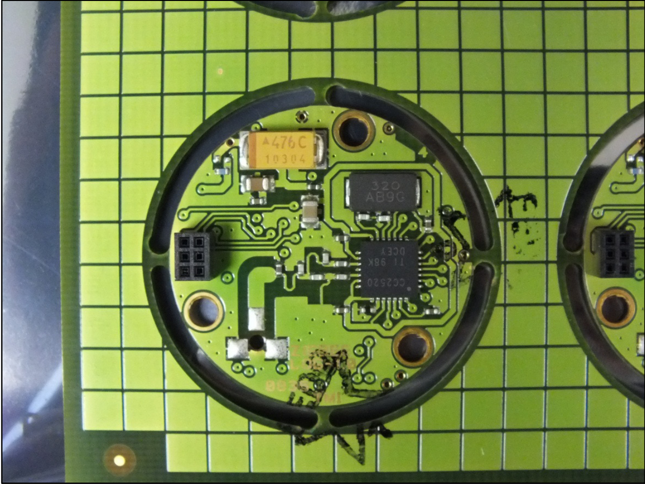
Figure 4: Radio Board Bottom View
