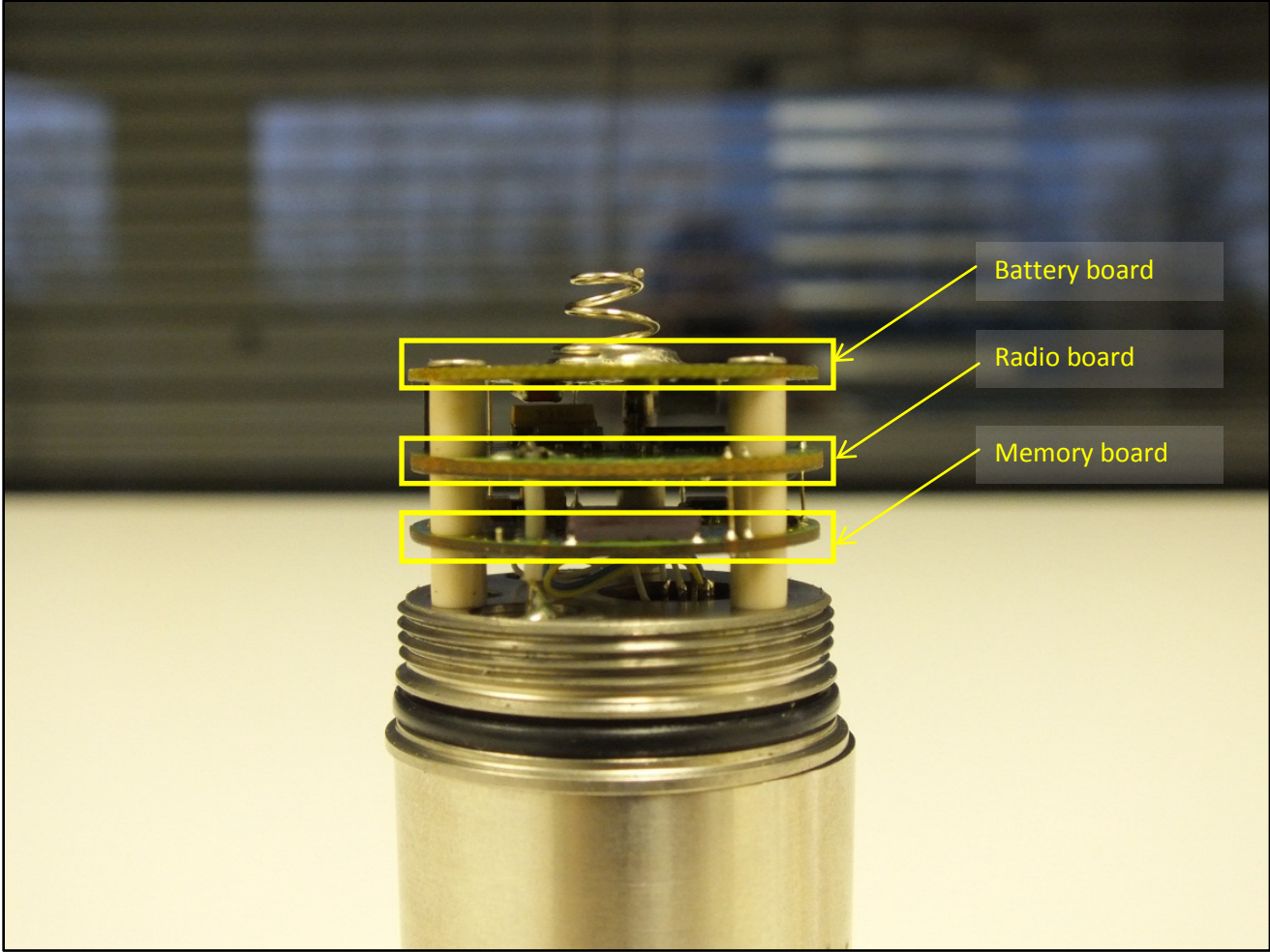
Figure 7: Final Assembly of the Circuit Boards in Data Logger with Battery Case Removed
