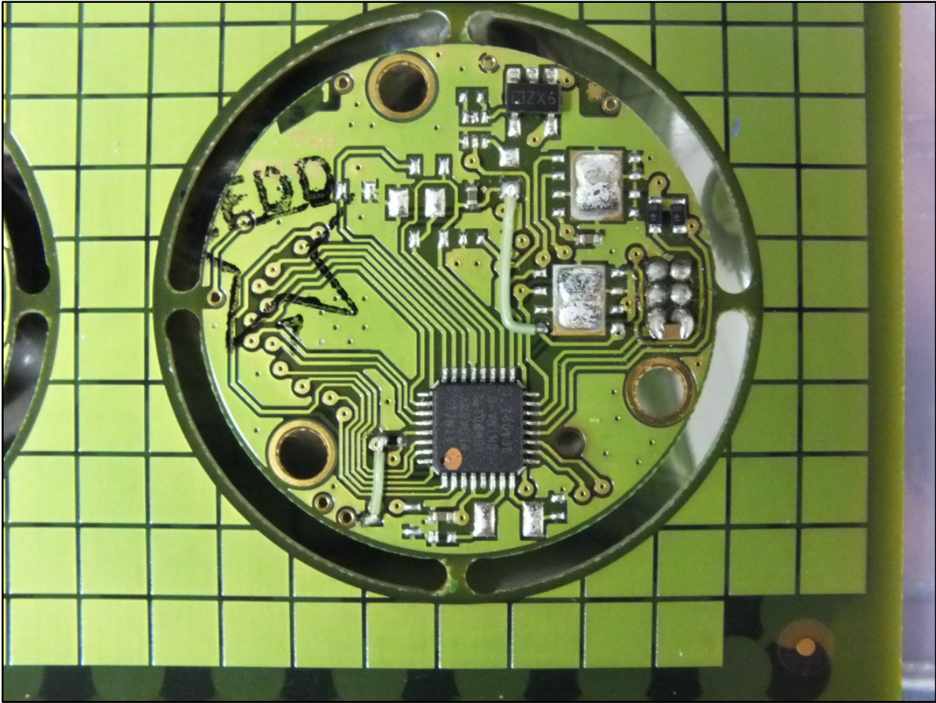
Figure 3: Radio Board Top View
