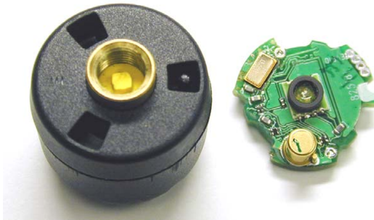
Bottom View of Circuit Board
