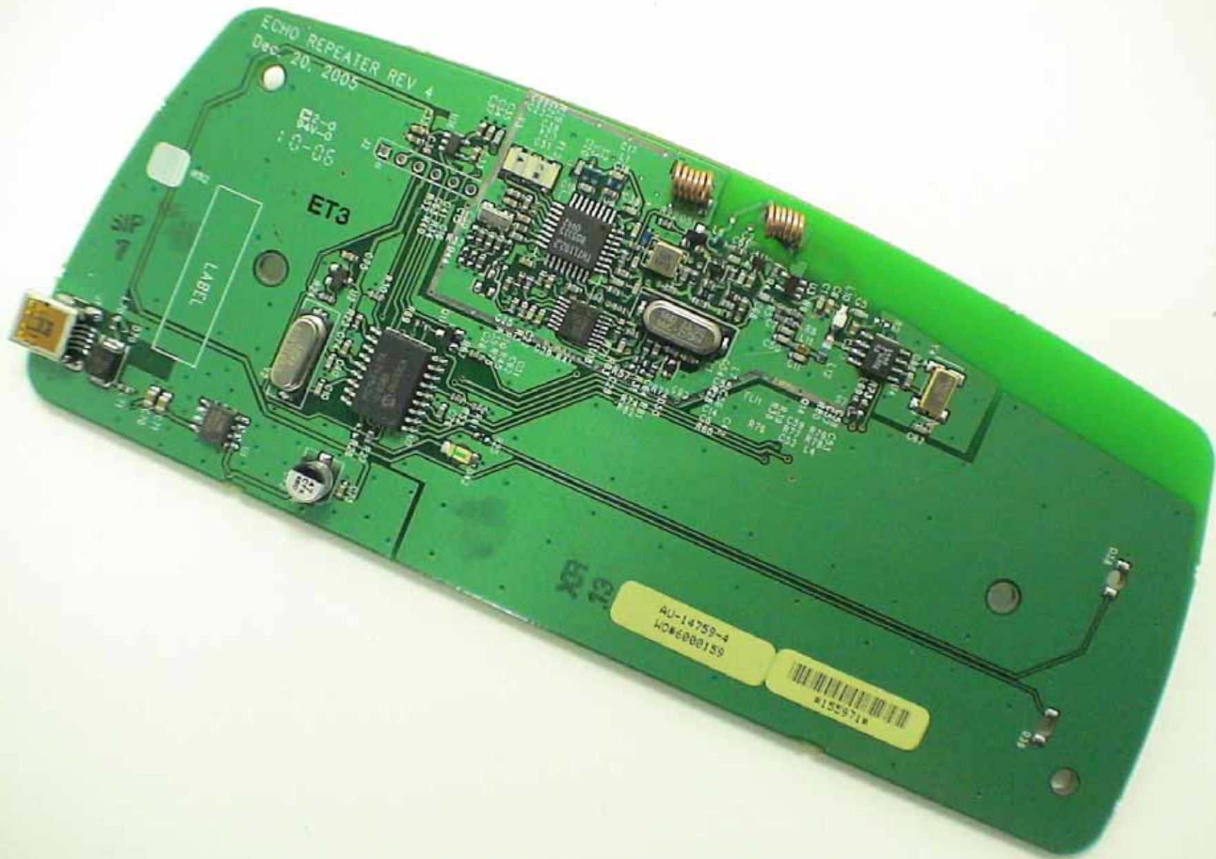
PCB (top)
