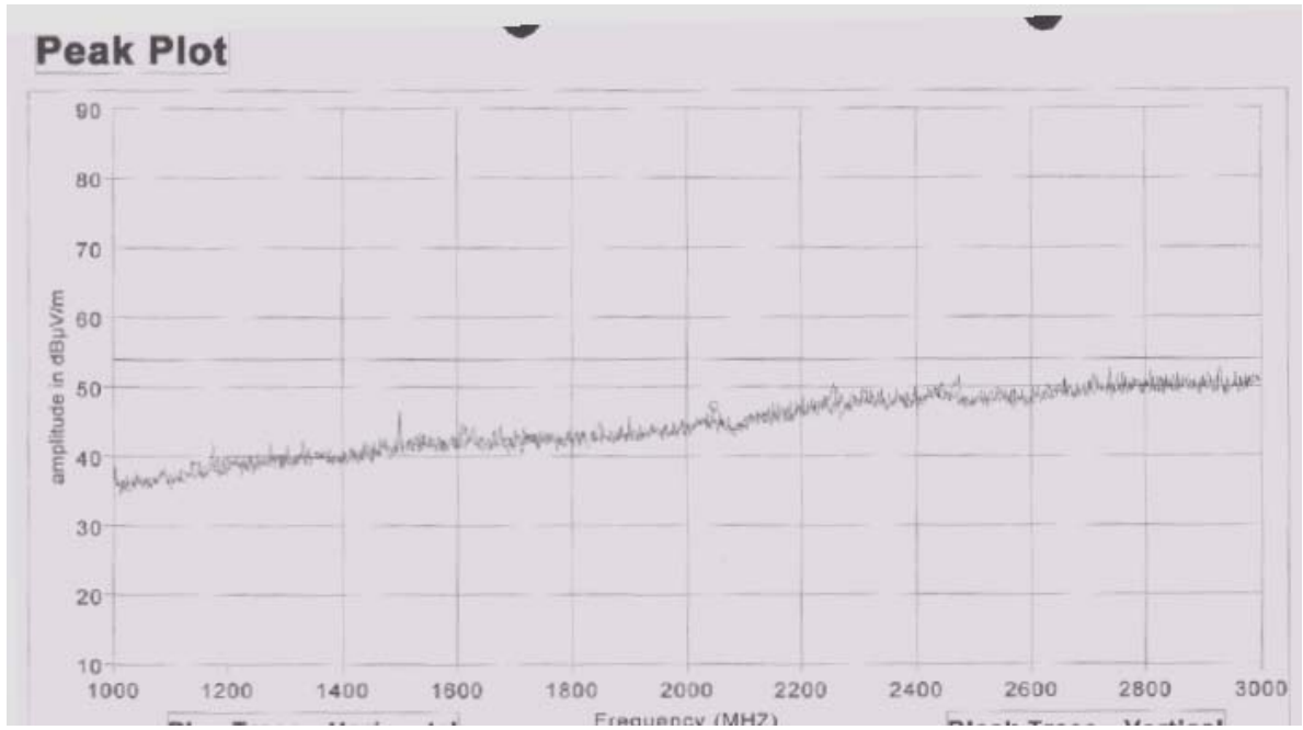
Channel 11 @ 802.11g 54Mbps (1GHz-3GHz)
