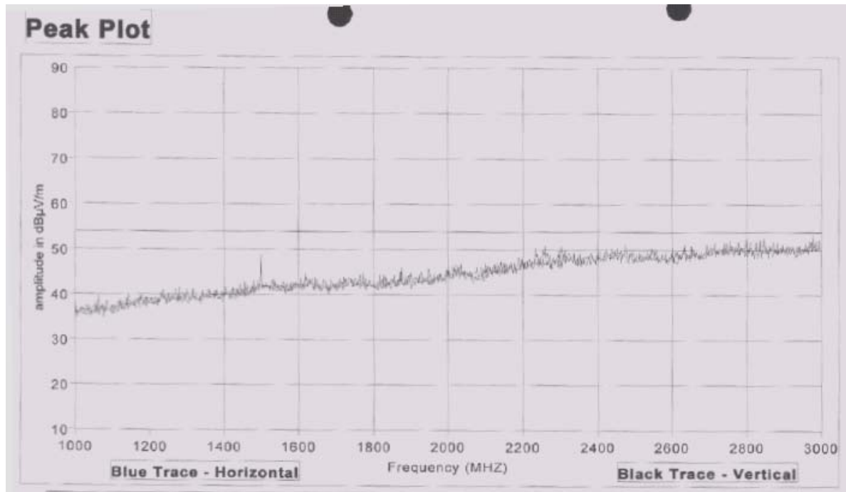
Channel 13 @ 802.11b 11Mbps (1GHz-3GHz)
