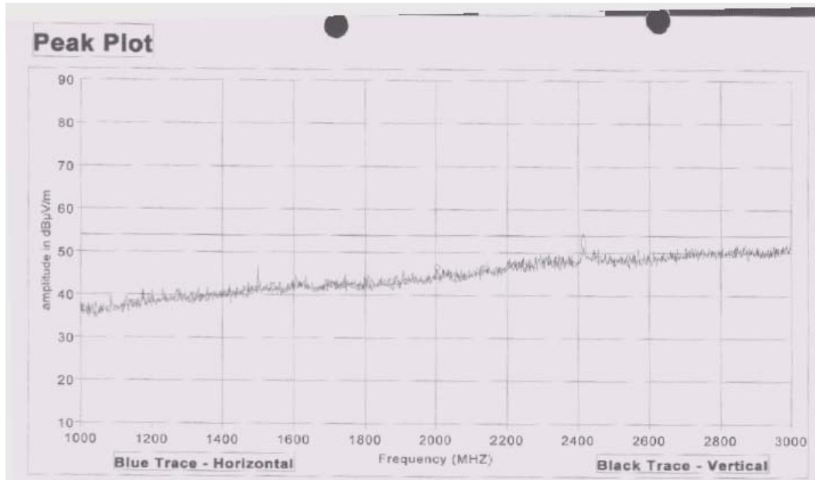
Channel 1 @ 802.11b 11Mbps (1GHz-3GHz)
