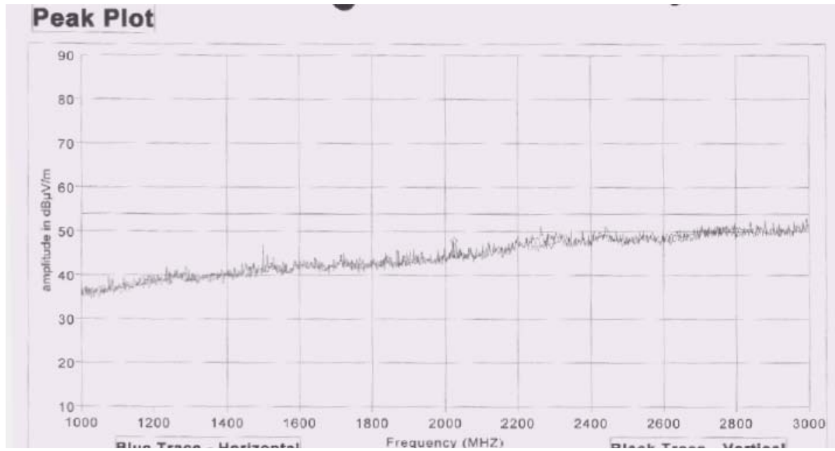
Channel 7 @ 802.11b 11Mbps (1GHz-3GHz)
