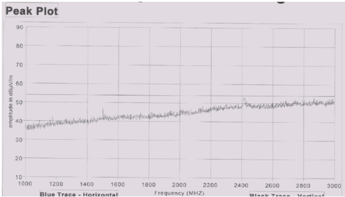
Channel 1 @ 802.11g 54Mbps (1GHz-3GHz)
