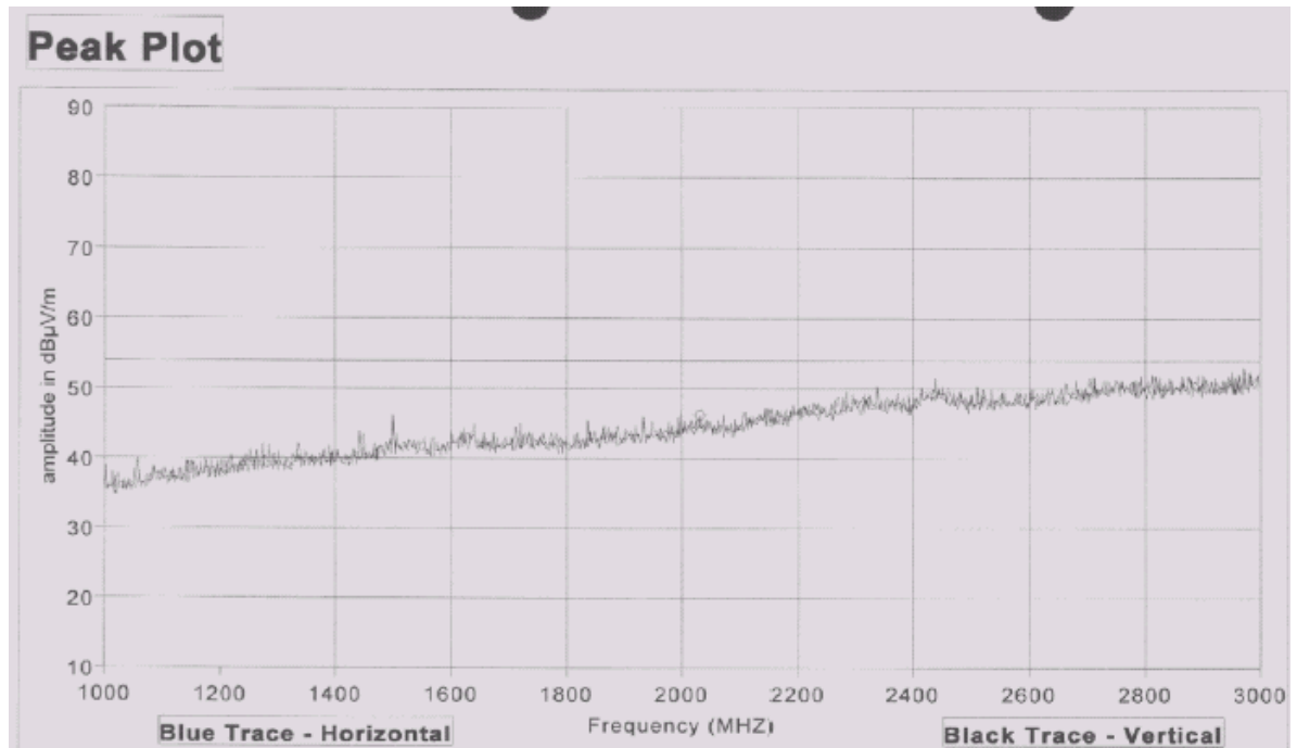
Channel 7 @ 802.11g 54Mbps (1GHz-3GHz)
