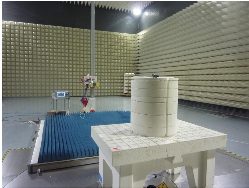
Figure 3: Test Setup for 1 GHz to 18 GHz (Rear View)
