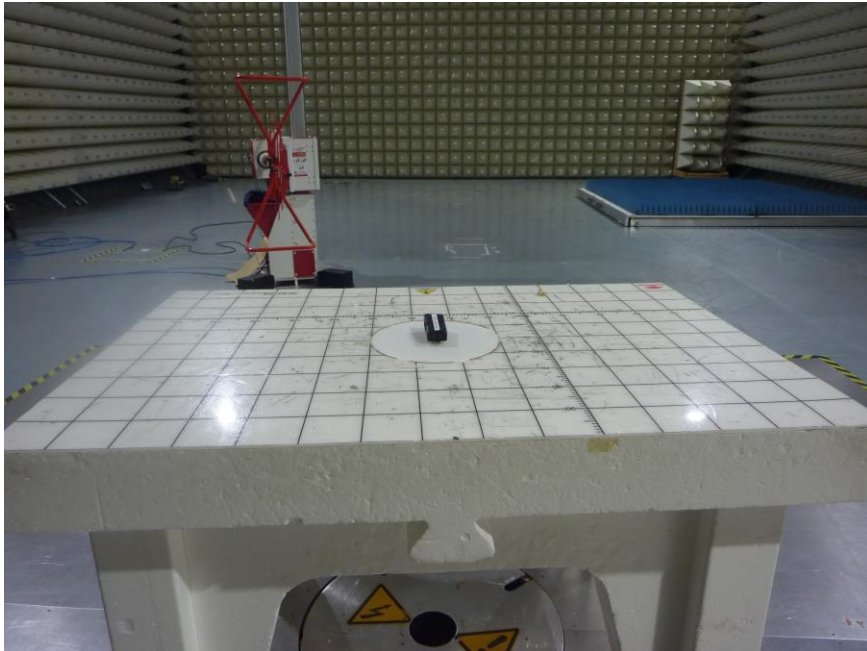
Figure 1: Test Setup for 30 MHz to 1 GHz (Rear View)
