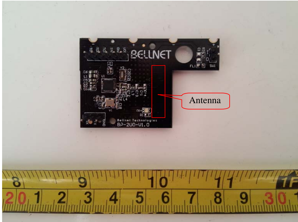
EUT –Bottom View (BN-BP200)
