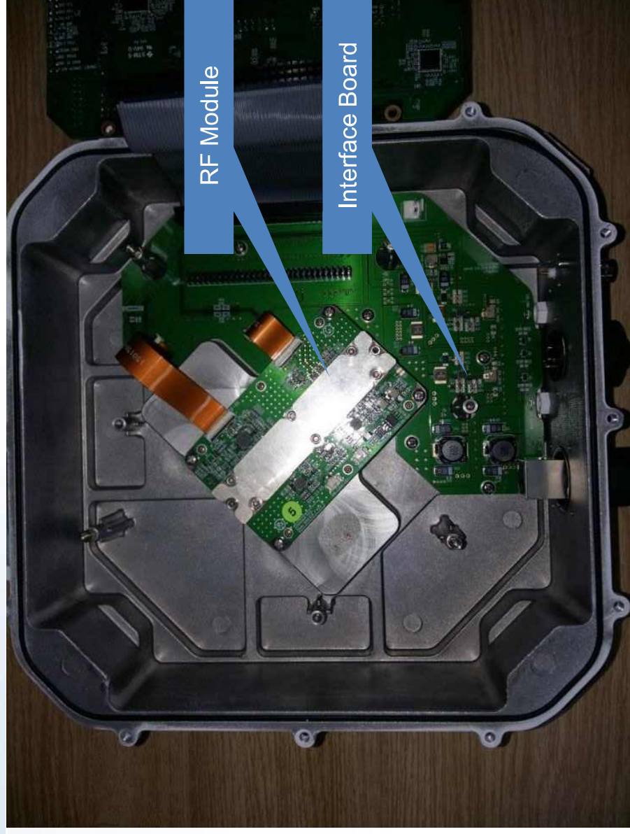
Internal photo of ODU with service compartment removed from modem board
