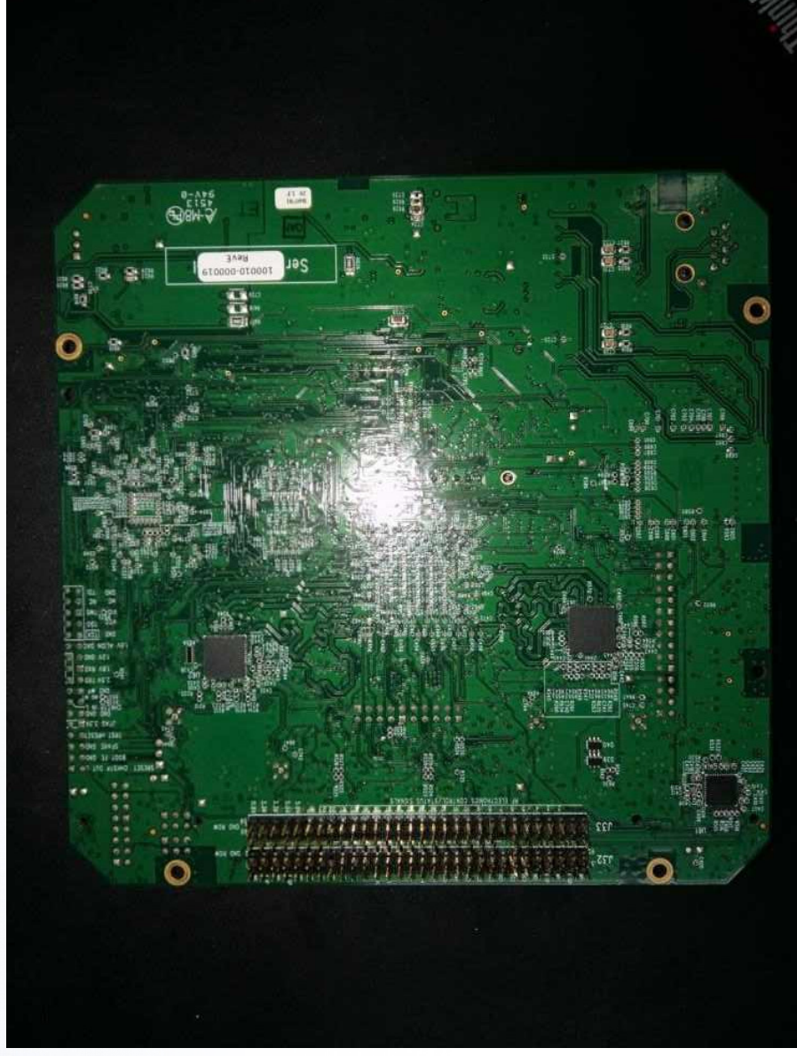
Photo of modem board - bottom view
