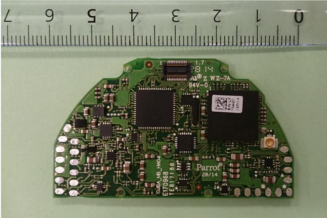
Picture 1 : Mother board front view
