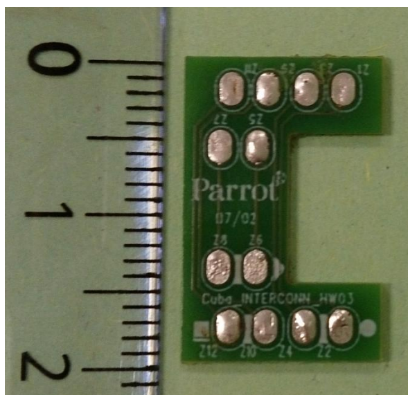
Picture 5 : Cuba interconn front view
