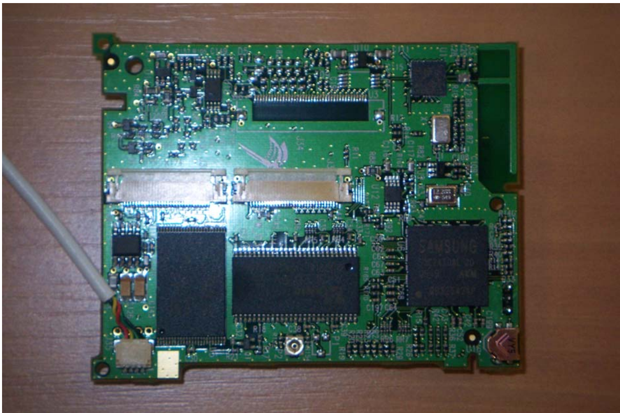
BOTTOM VIEW
