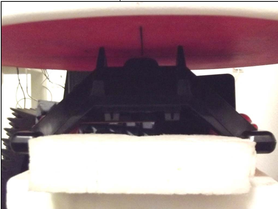
Photo 12: DUT - test position bottom with 0mm distance
